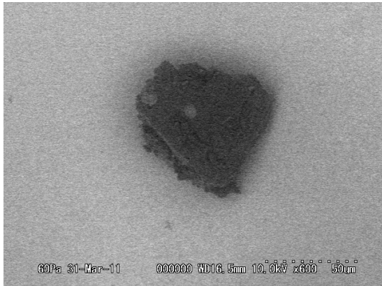
20110331/Au03SEM/BSE/S_2b_Z17mm_Tilt20deg.bmp
