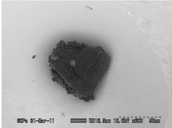
20110331/Au03SEM/BSE/S_2bfine_Z17mm_Tilt20deg.bmp
