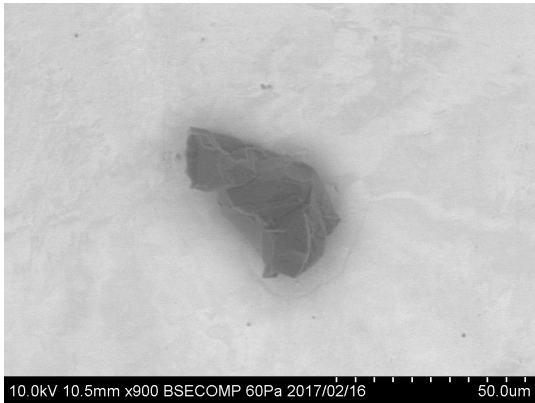
20170216/Au12_SEM/image/07_Au12s19_bse.bmp
