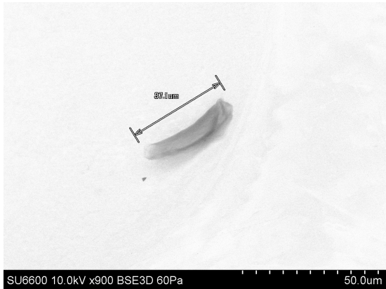
20121112/Au11_SEM/image/11_CV-49_BSE_scaled.bmp
