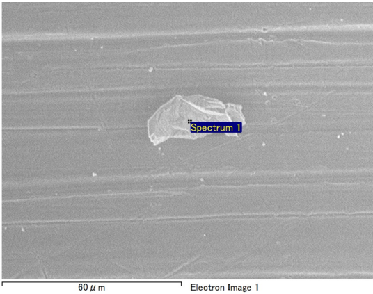
Spectrum 1
