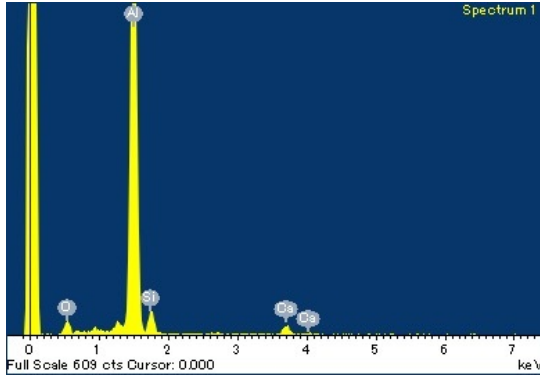
Spectrum 1
