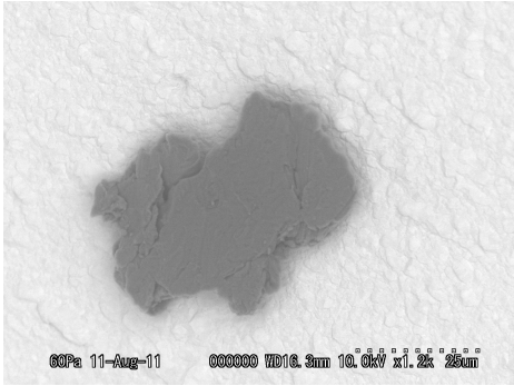
20110811/Au08SEM/BSE/03_Au08_outside.bmp
