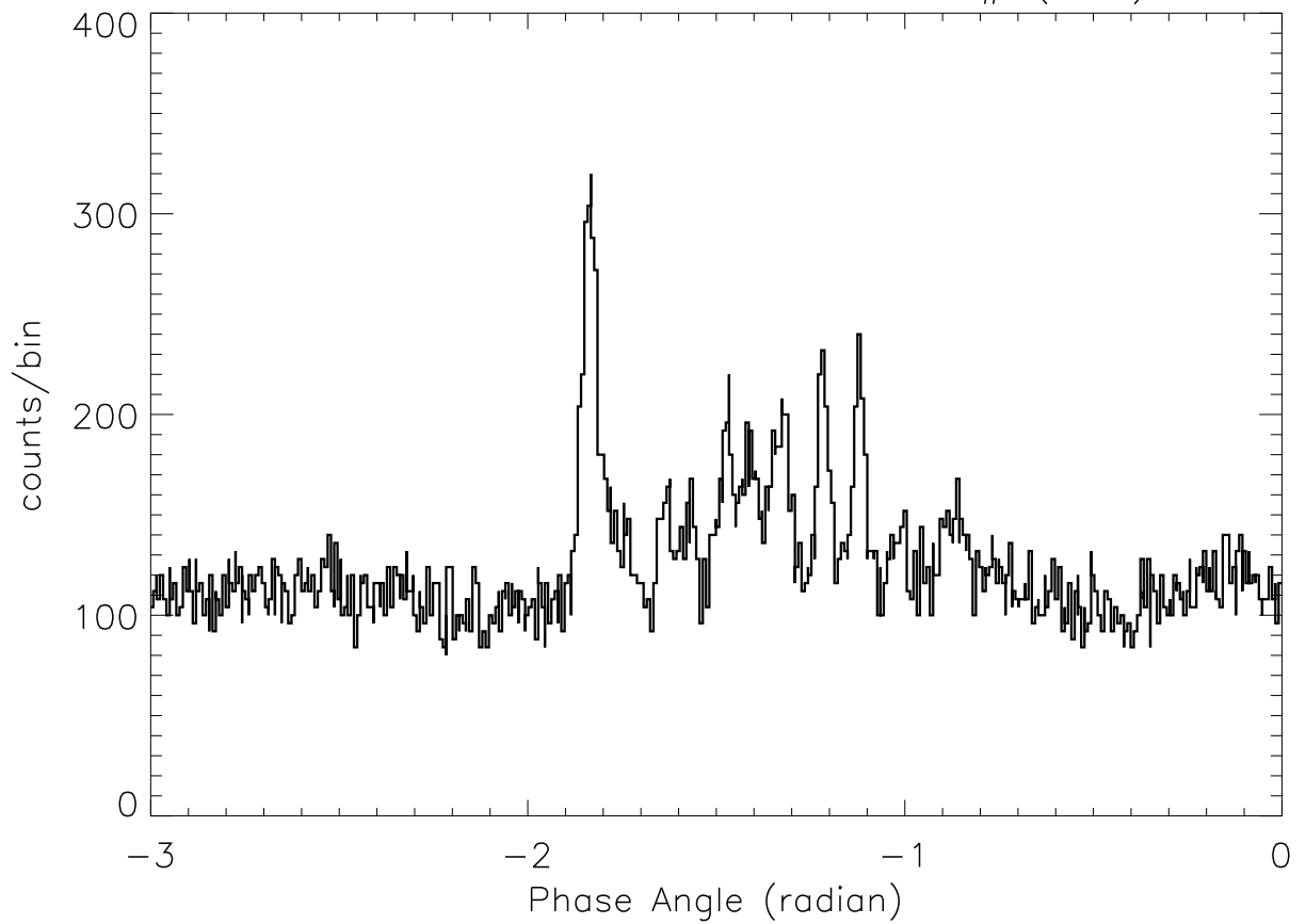
SOX2: 23: 6:31 – 23: 6:39 SP# ( 84)
