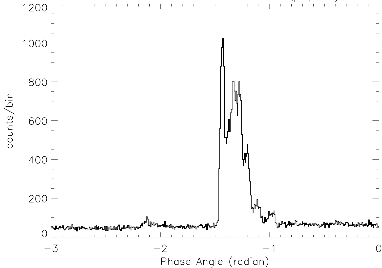
SOX2: 23: 0:51 – 23: 1: 0 SP# ( 45)
