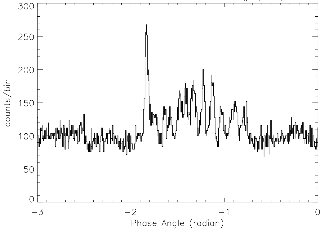
SOX2: 23: 8:41 – 23: 8:50 SP# ( 99)
