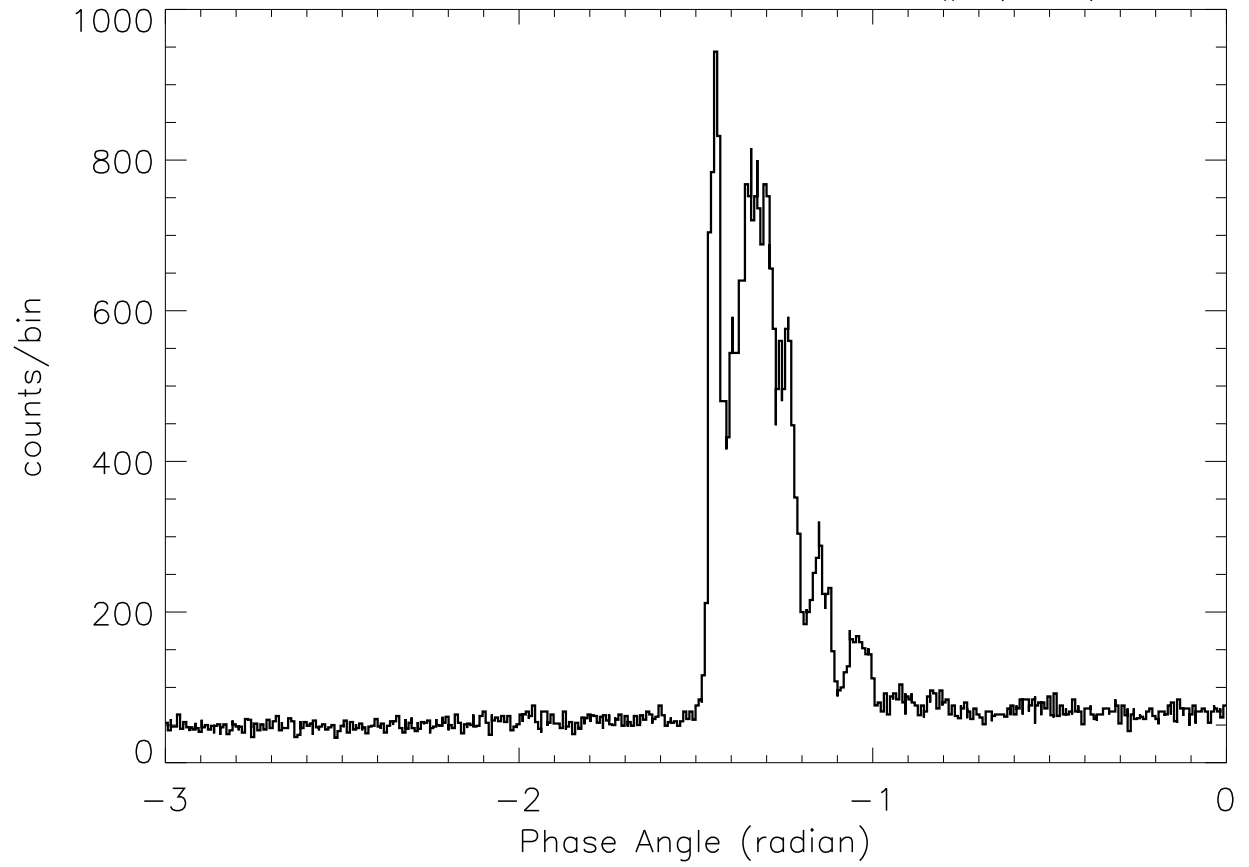
SOX2: 23: 9:25 – 23: 9:33 SP# (104)
