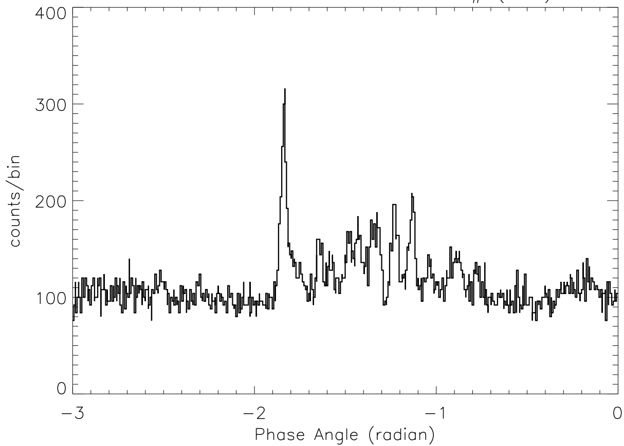
SOX2: 23: 7:58 – 23: 8: 6 SP# ( 94)
