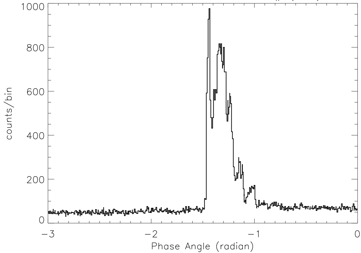
SOX2: 23: 8:41 – 23: 8:50 SP# ( 99)
