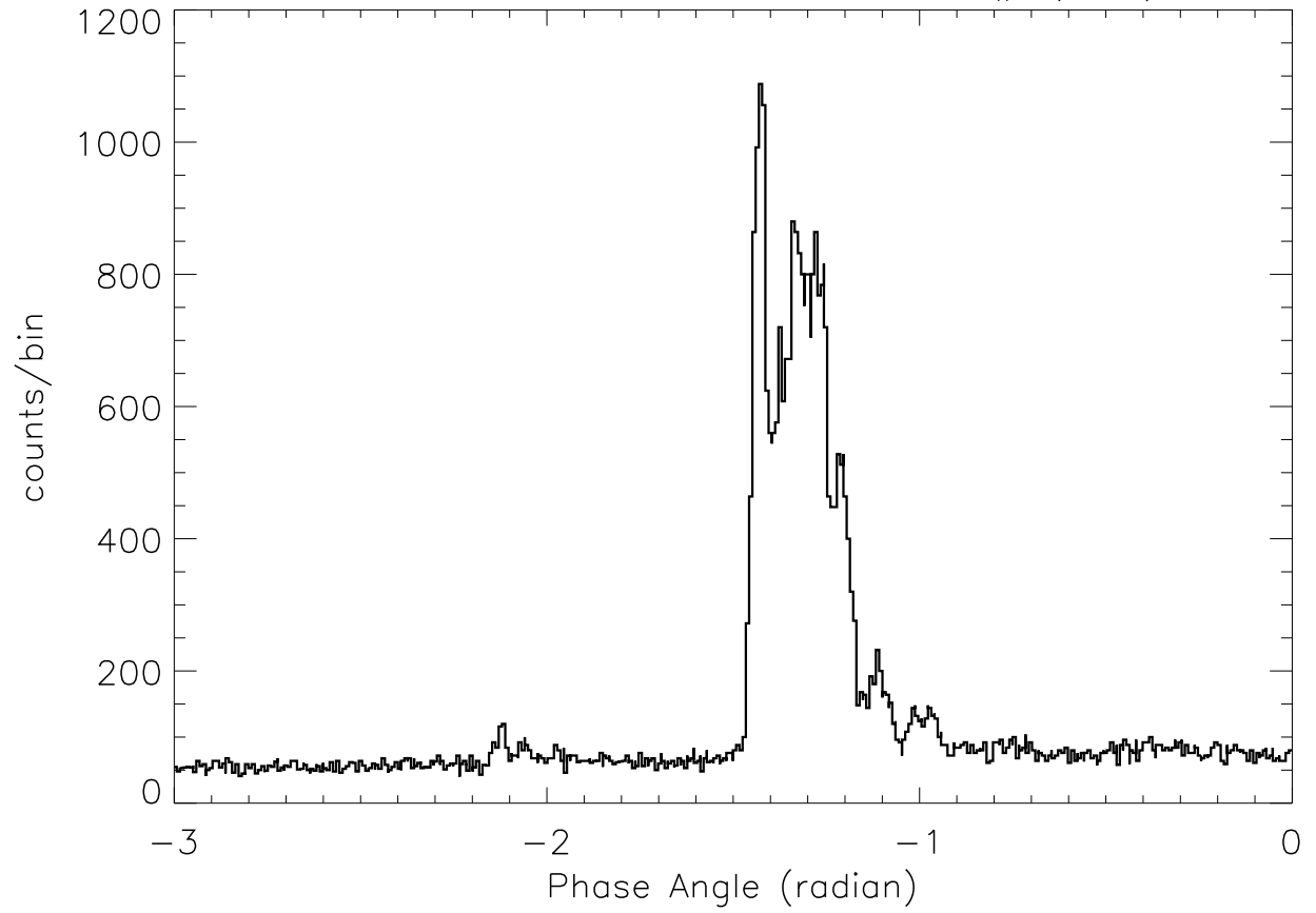
SOX2: 23: 1:44 – 23: 1:52 SP# ( 51)
