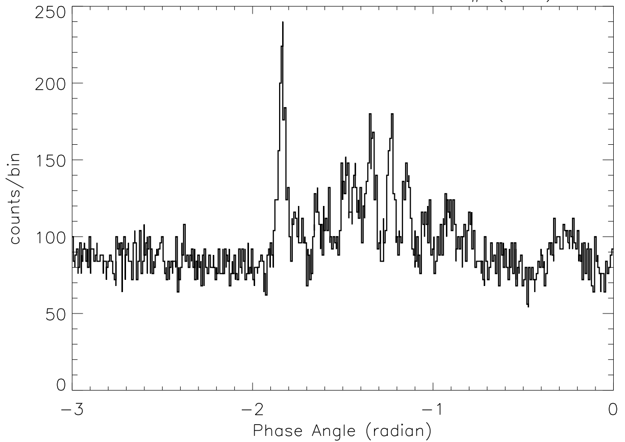
SOX2: 23:10:34 – 23:10:43 SP# (112)
