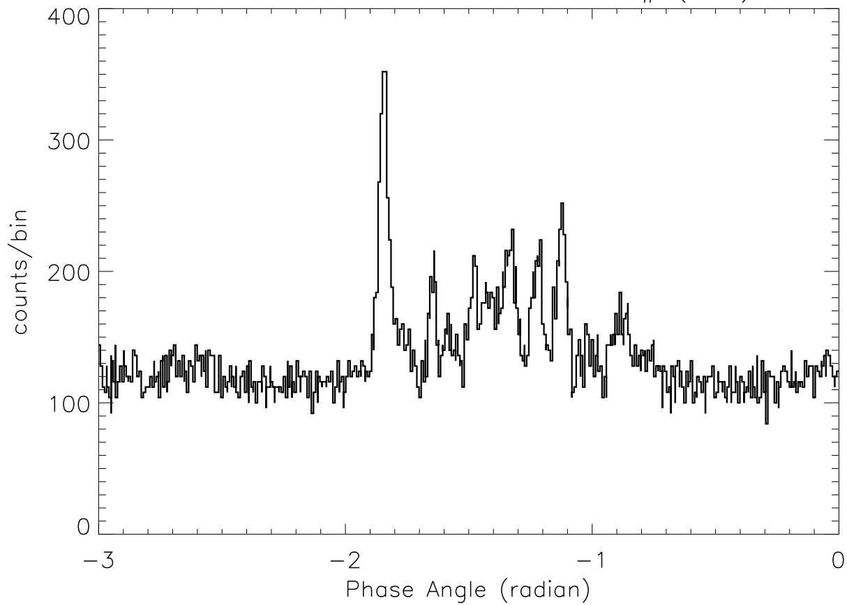
SOX2: 23: 5:12 – 23: 5:21 SP# ( 75)
