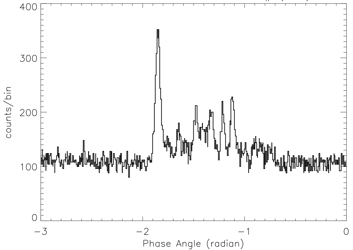
SOX2: 23: 2:18 – 23: 2:27 SP# ( 55)
