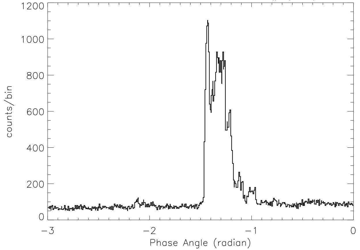
SOX2: 23: 3:11 – 23: 3:19 SP# ( 61)
