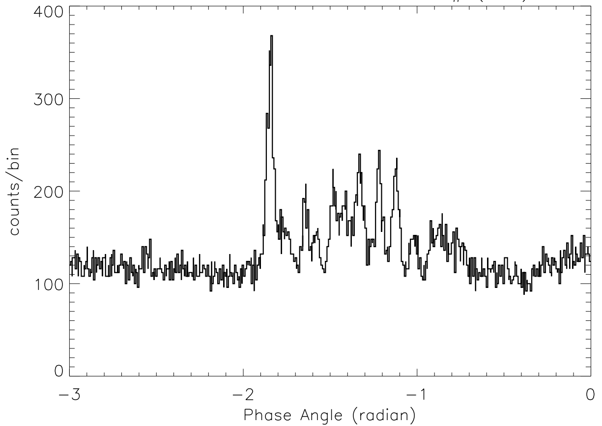
SOX2: 23: 5:21 – 23: 5:30 SP# ( 76)
