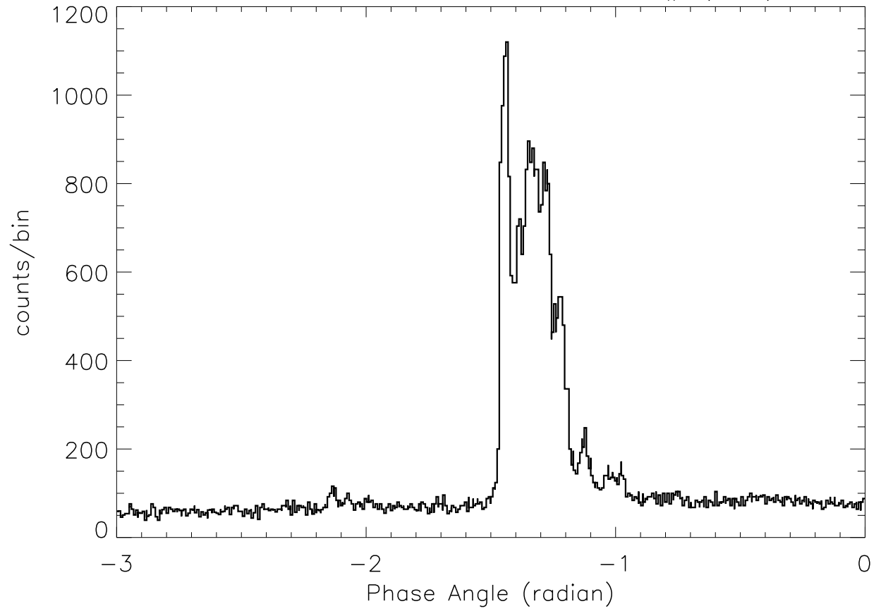
SOX2: 23: 2:18 – 23: 2:27 SP# ( 55)
