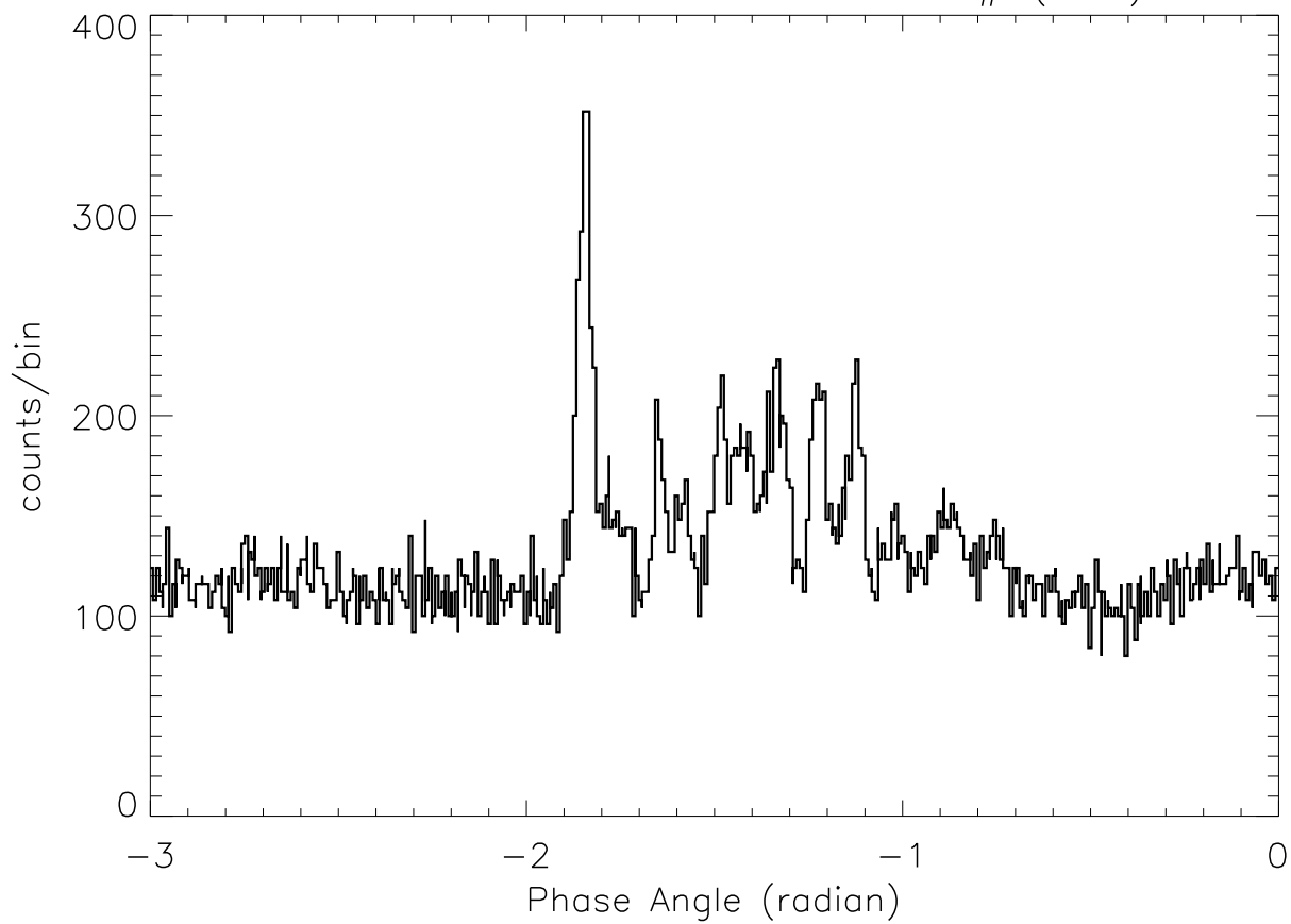
SOX2: 23: 5:38 – 23: 5:47 SP# ( 78)
