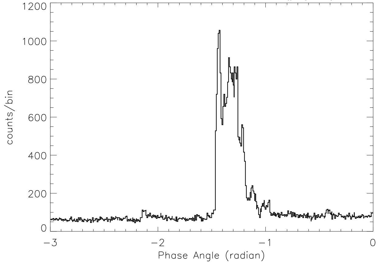
SOX2: 23: 2:10 – 23: 2:18 SP# ( 54)
