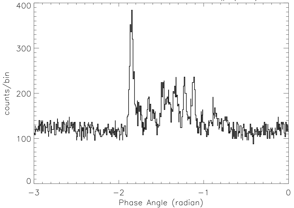
SOX2: 23: 4:11 – 23: 4:20 SP# ( 68)
