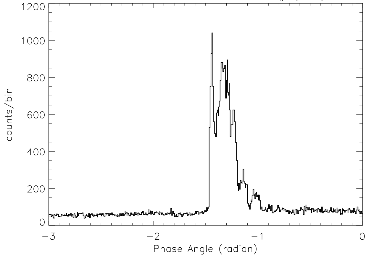
SOX2: 23: 7:23 – 23: 7:31 SP# ( 90)
