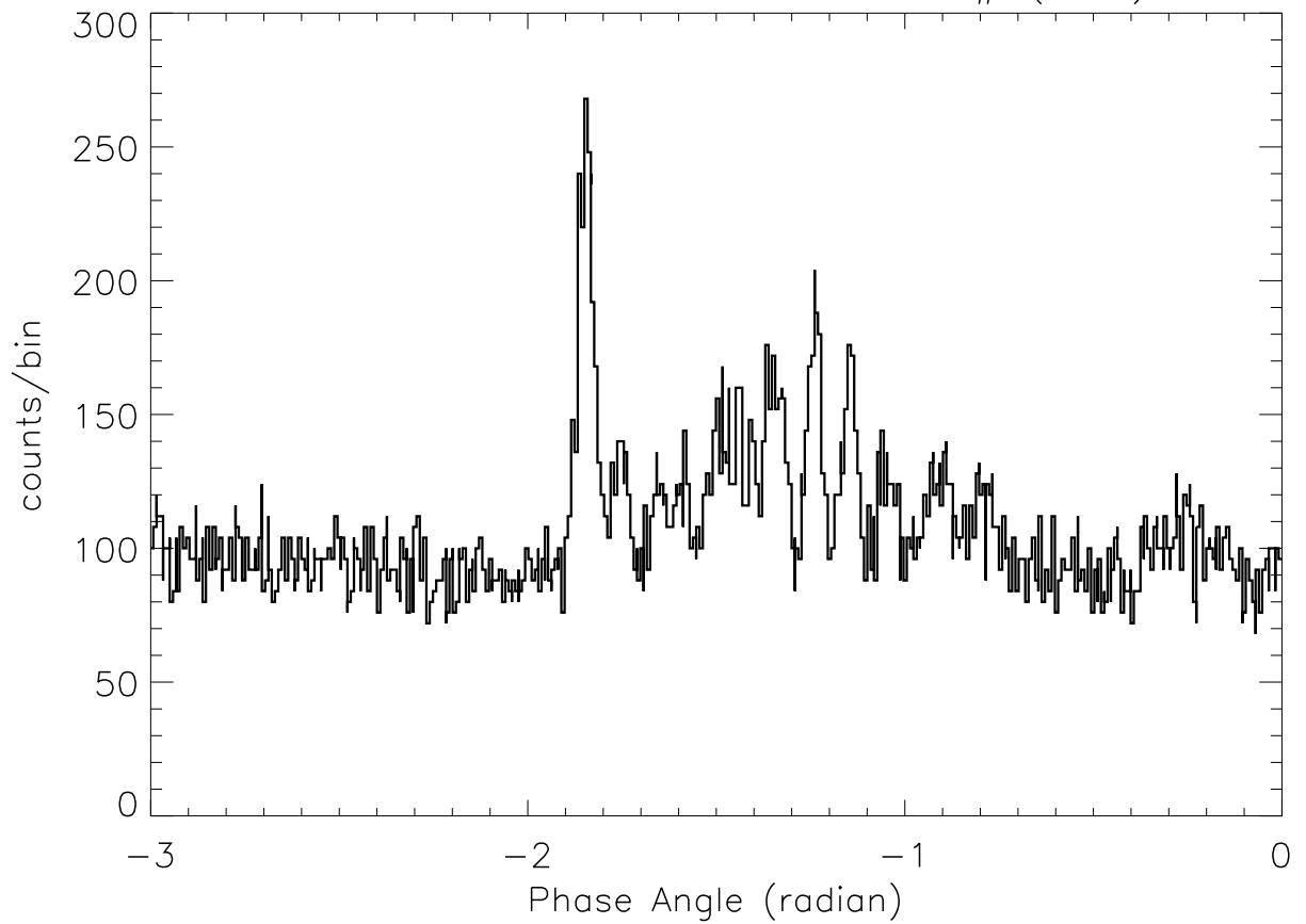
SOX2: 23: 9: 7 – 23: 9:16 SP# (102)
