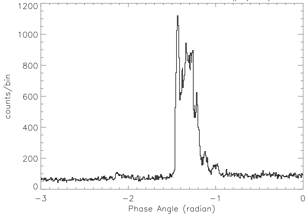
SOX2: 23: 2:53 – 23: 3: 2 SP# ( 59)
