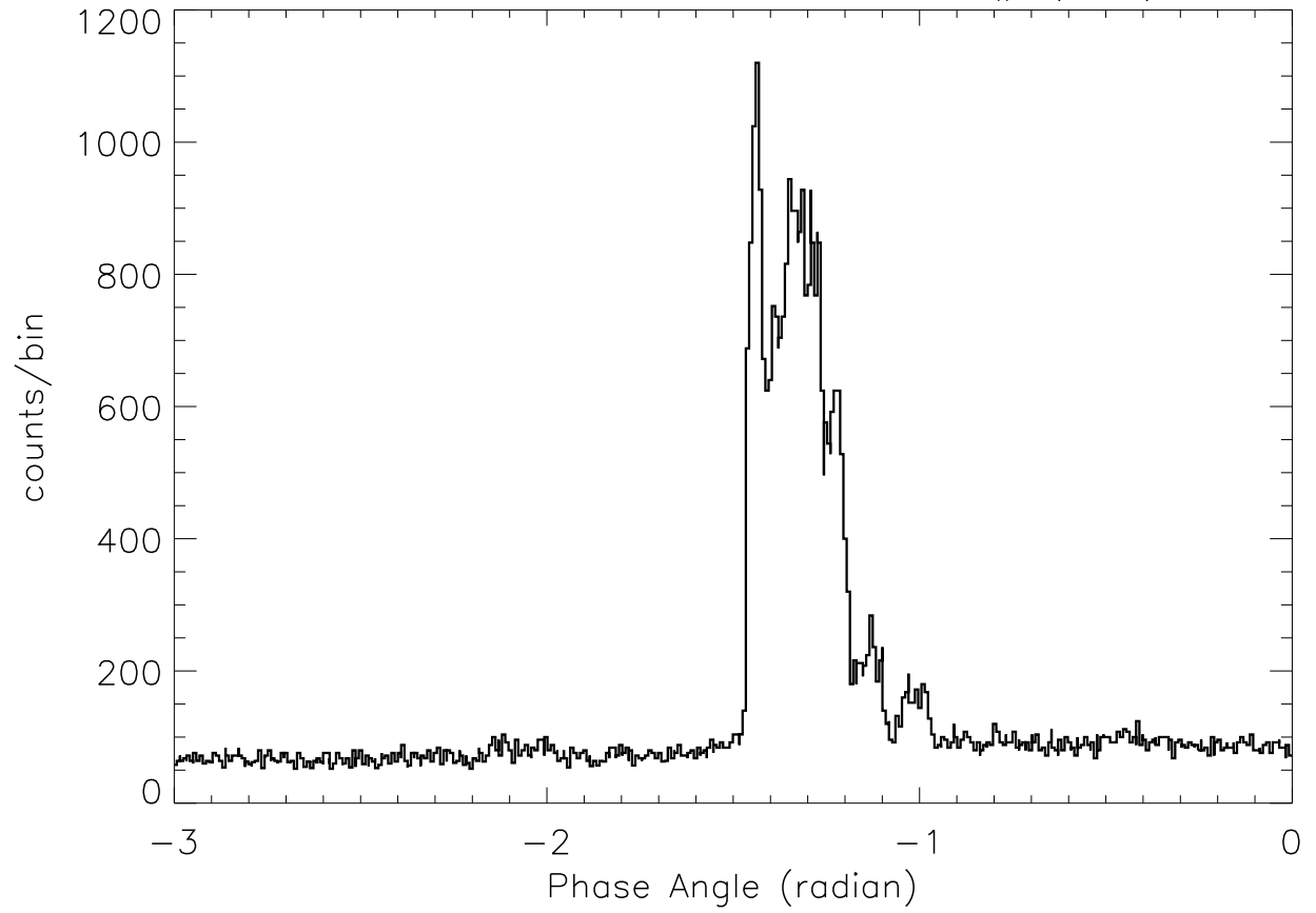
SOX2: 23: 4:46 – 23: 4:55 SP# ( 72)
