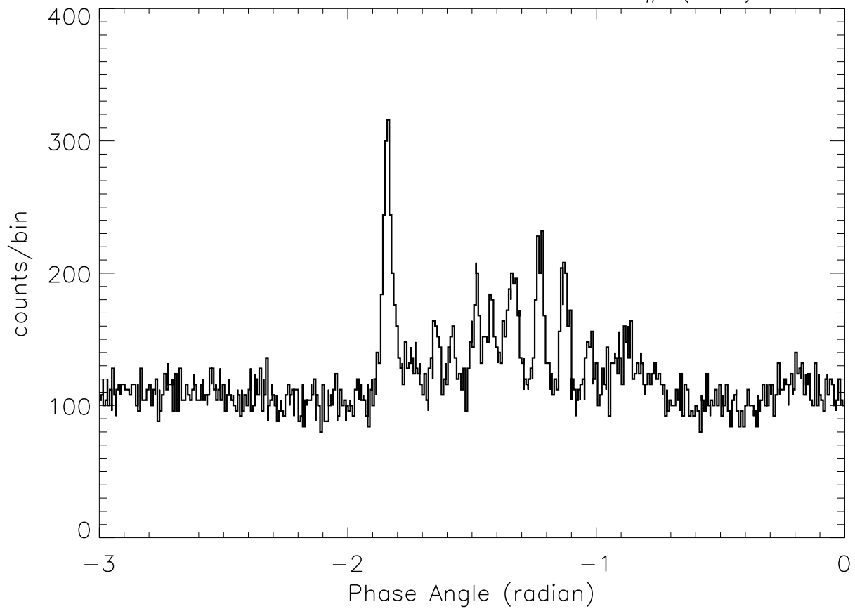
SOX2: 23: 7: 5 – 23: 7:14 SP# ( 88)
