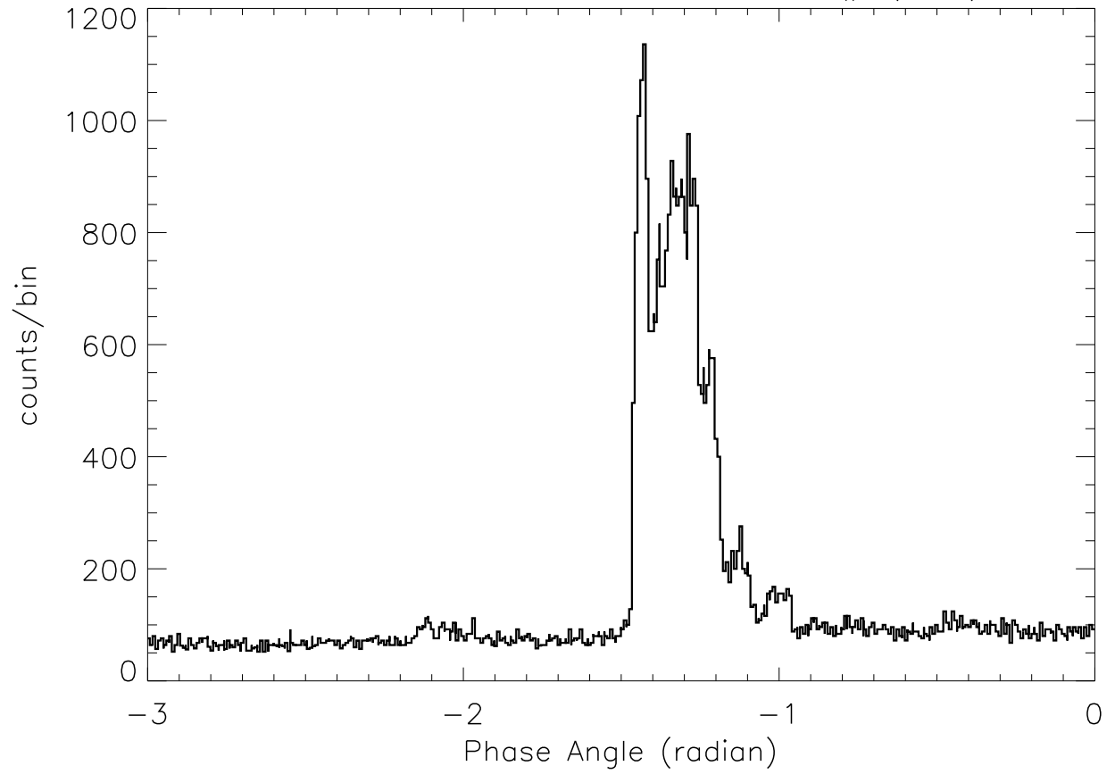
SOX2: 23: 3:19 – 23: 3:28 SP# ( 62)
