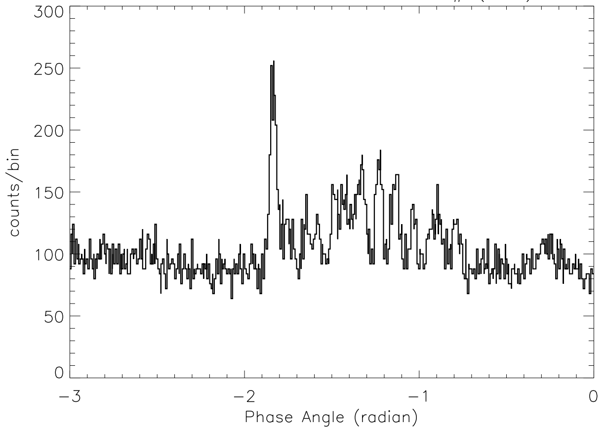
SOX2: 23: 9:33 – 23: 9:42 SP# (105)
