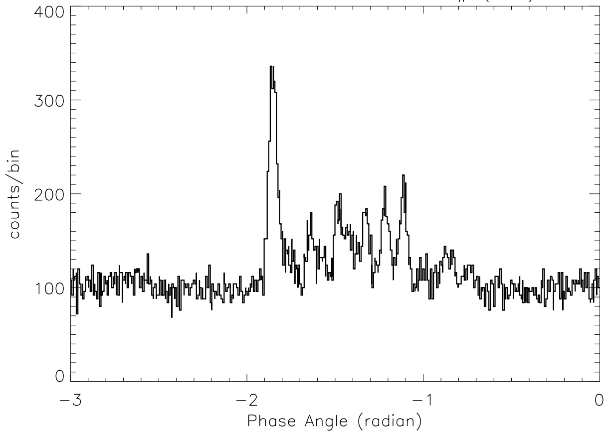
SOX2: 23: 1:52 - 23: 2: 1 SP# ( 52)
