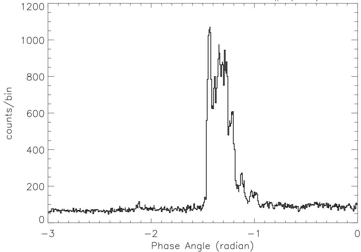
SOX2: 23: 4: 3 - 23: 4:11 SP# ( 67)
