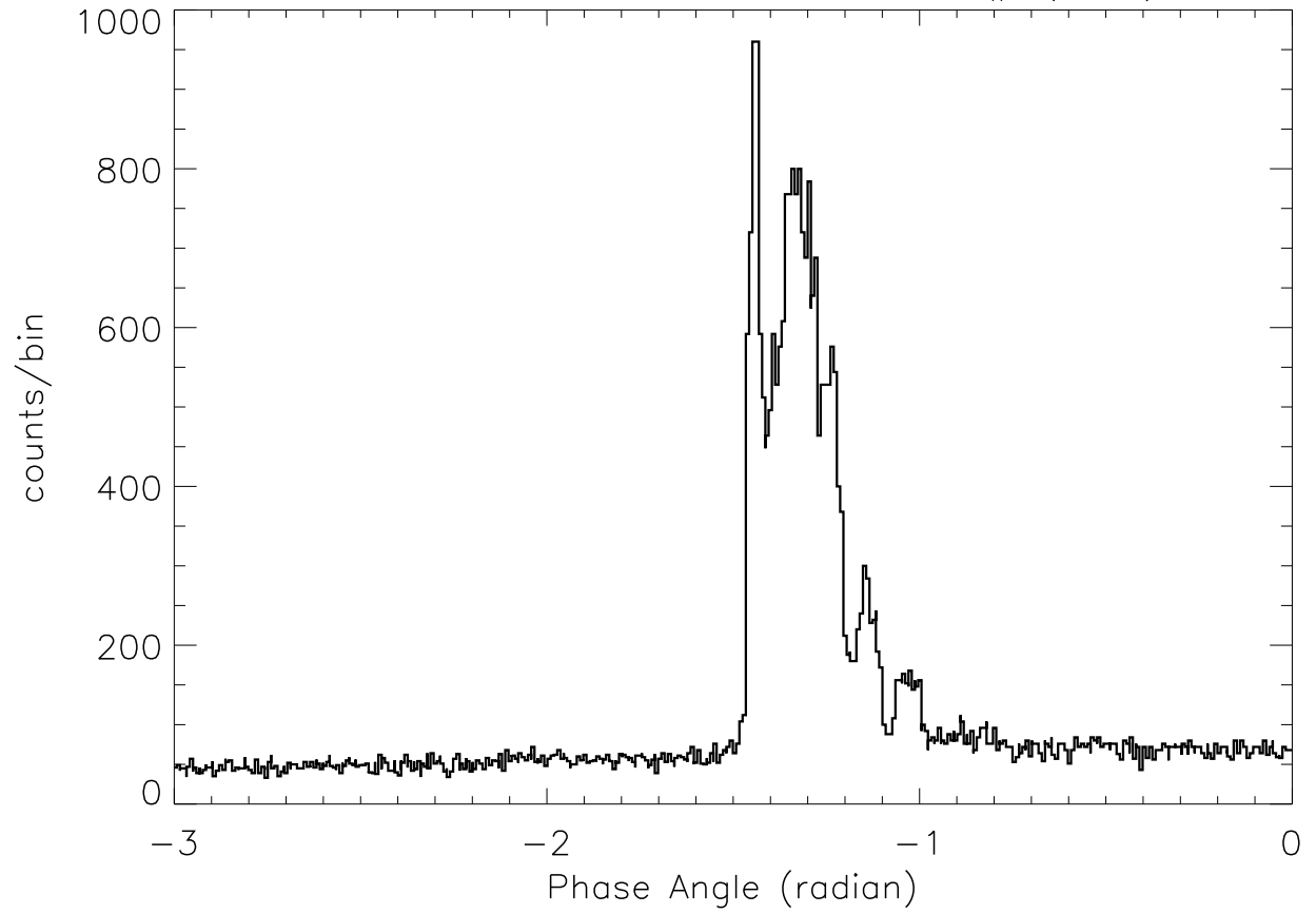
SOX2: 23: 8:58 – 23: 9: 7 SP# (101)
