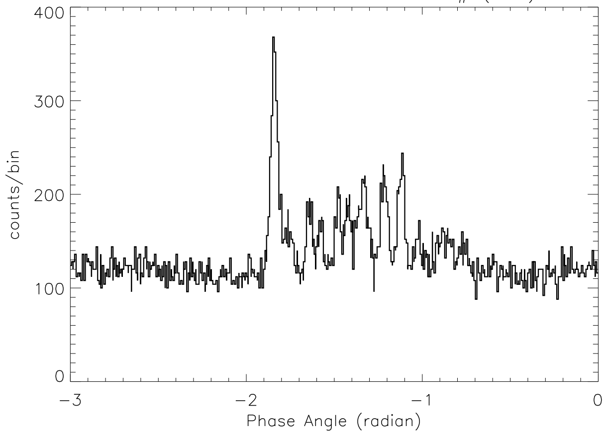
SOX2: 23: 5:30 – 23: 5:38 SP# ( 77)
