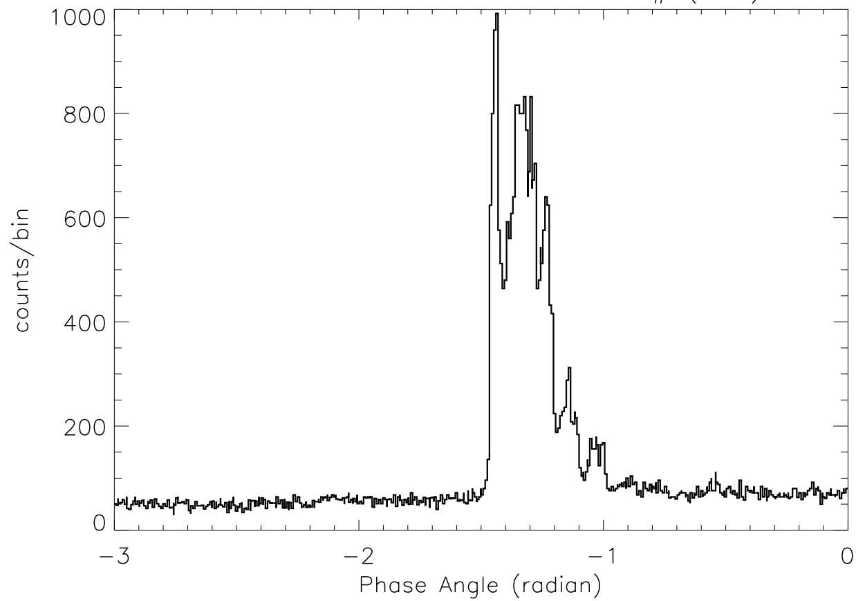
SOX2: 23: 8:24 – 23: 8:32 SP# ( 97)
