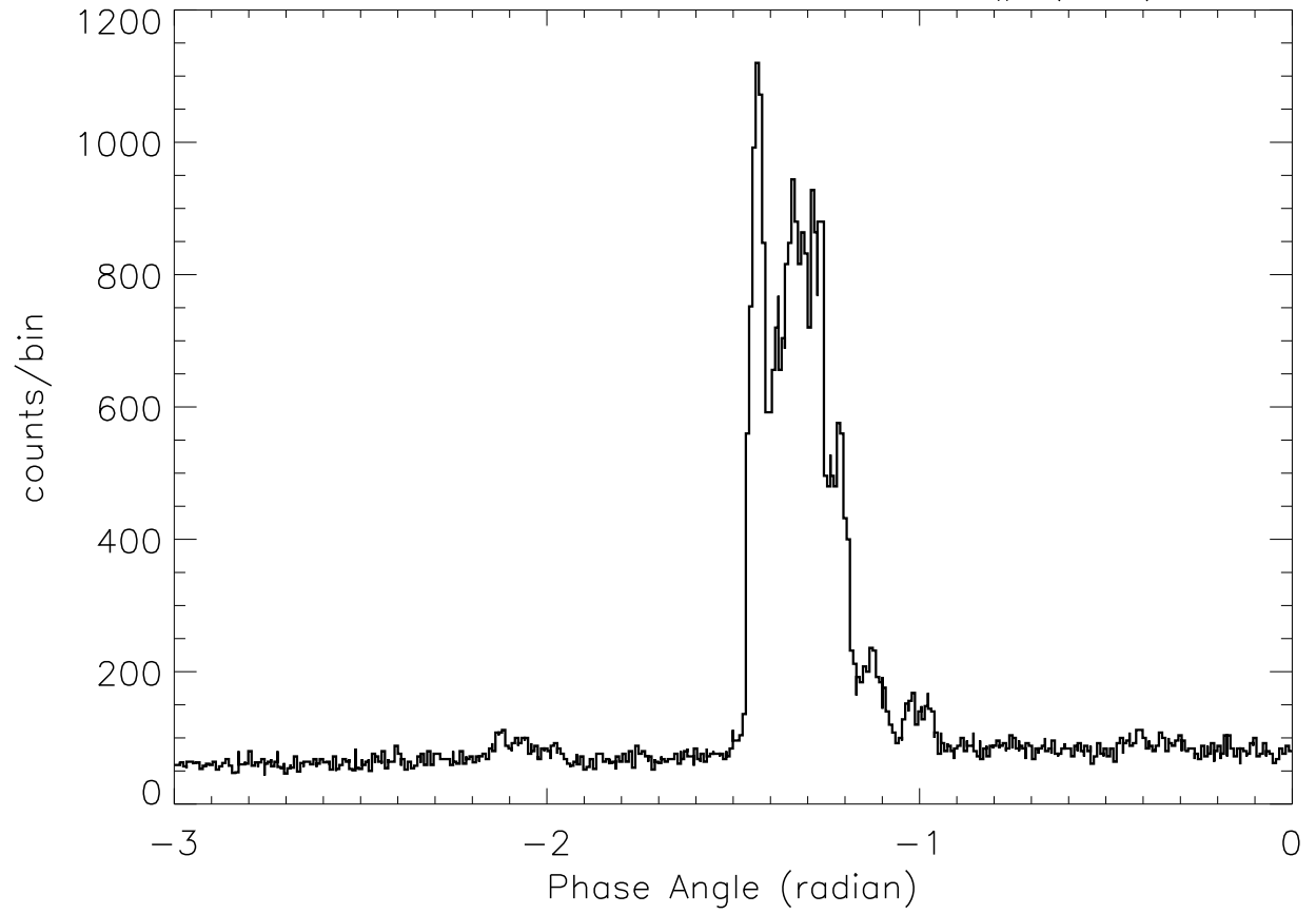
SOX2: 23: 2:27 – 23: 2:36 SP# ( 56)
