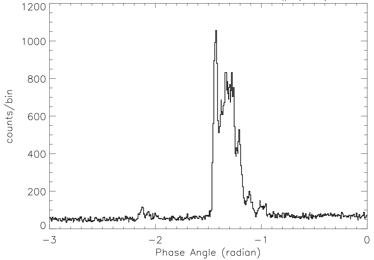
SOX2: 23: 1: 9 - 23: 1:18 SP# ( 47)
