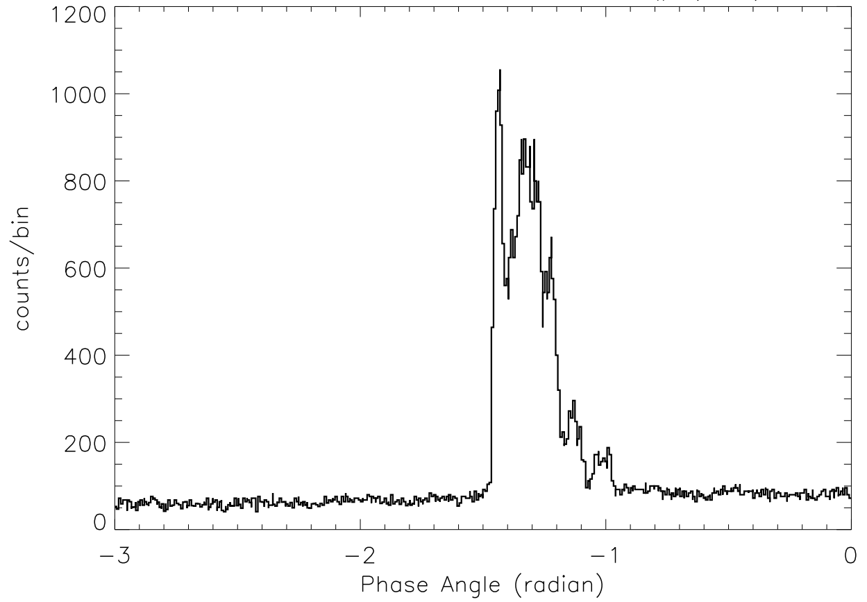
SOX2: 23: 6:22 – 23: 6:31 SP# ( 83)
