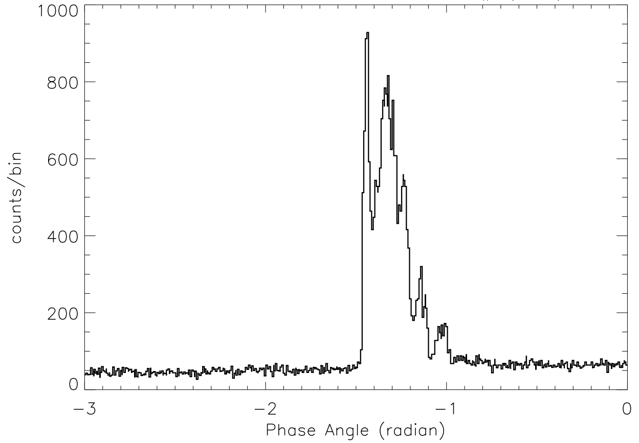
SOX2: 23: 9:51 – 23: 9:59 SP# (107)
