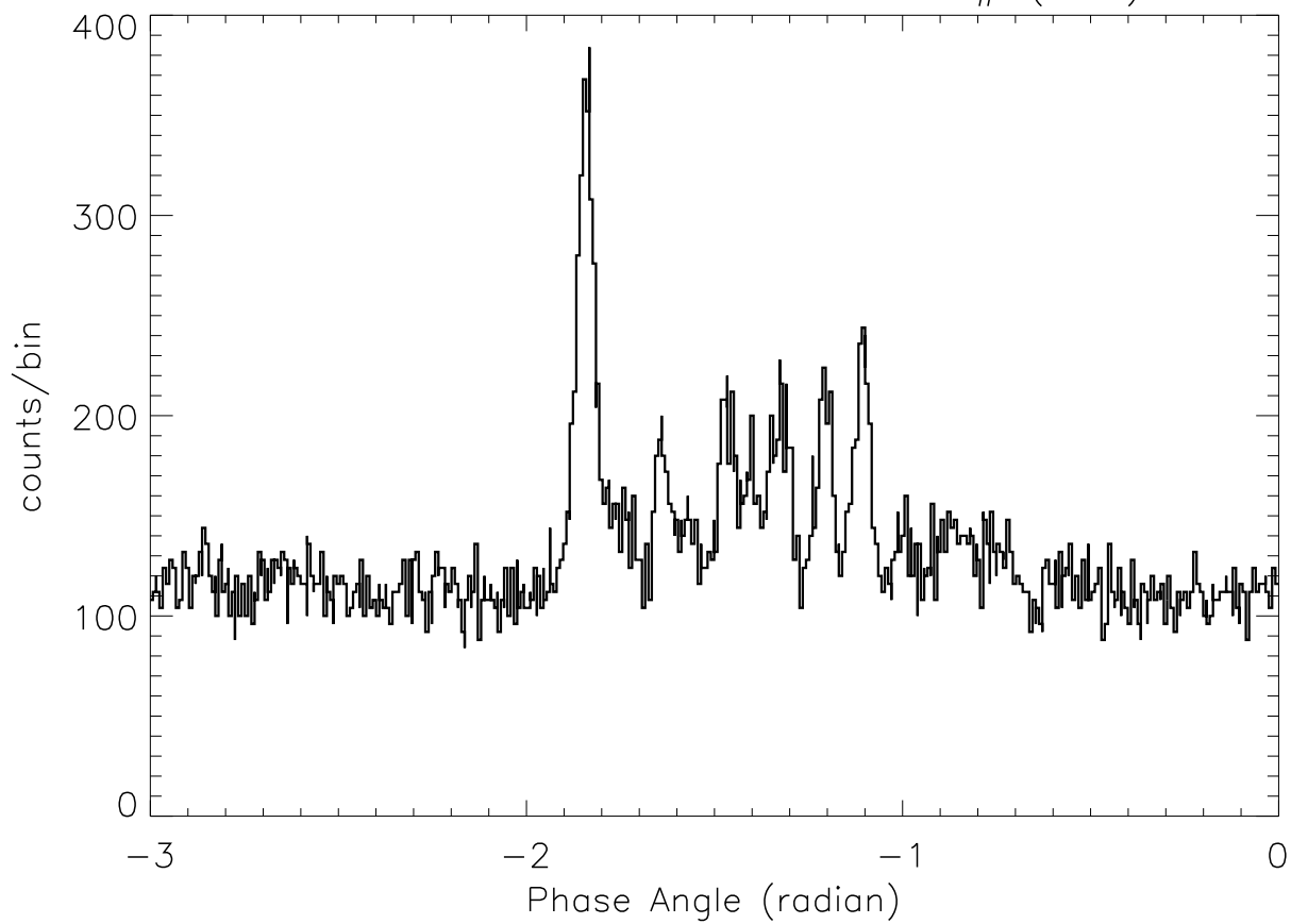
SOX2: 23: 2:53 – 23: 3: 2 SP# ( 59)
