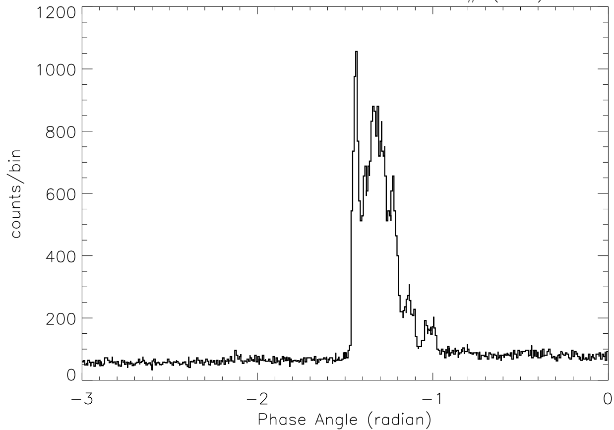
SOX2: 23: 6:57 – 23: 7: 5 SP# ( 87)
