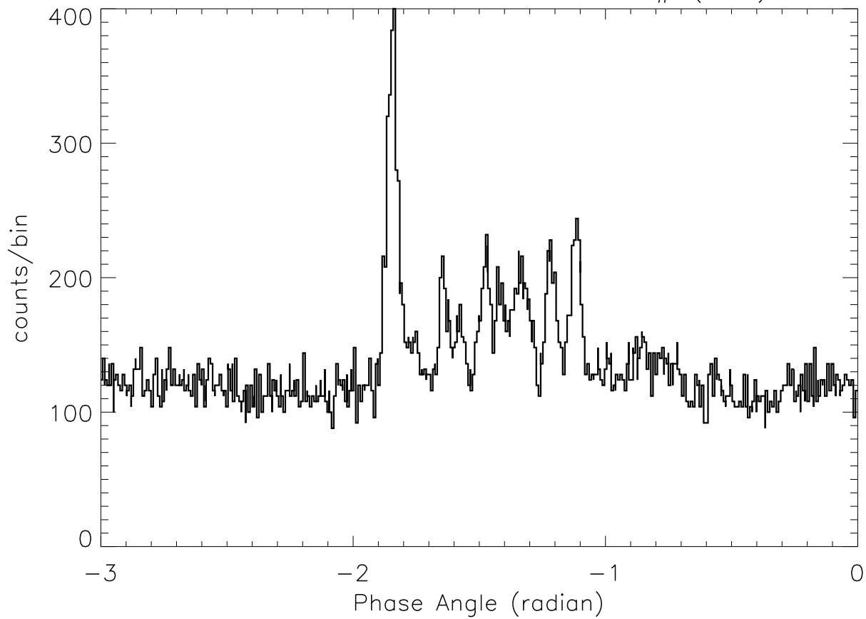
SOX2: 23: 3:37 – 23: 3:45 SP# ( 64)
