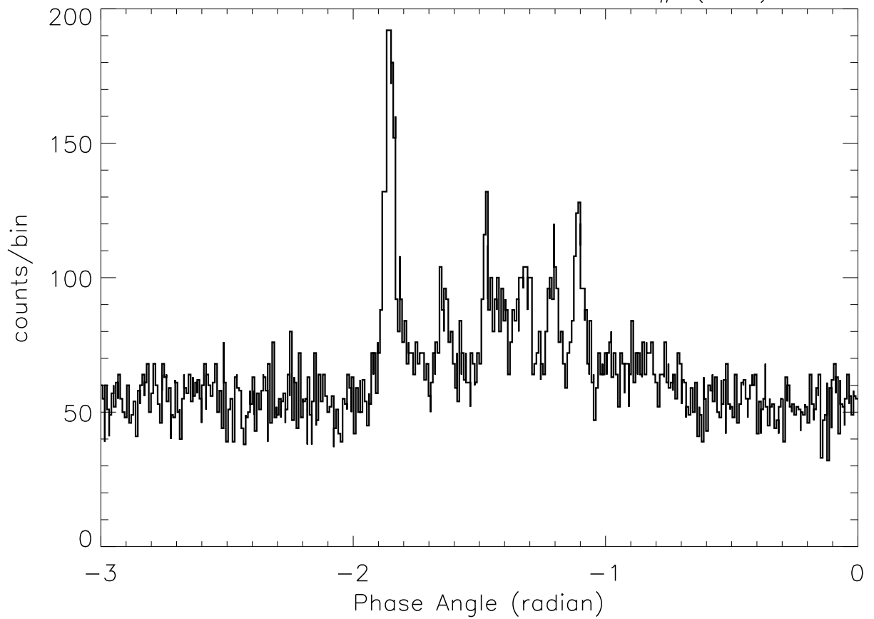
SOX2: 22:59: 7 – 22:59:16 SP# ( 33)
