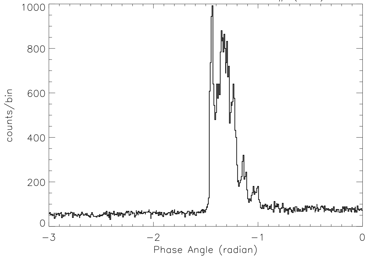
SOX2: 23: 7:58 – 23: 8: 6 SP# ( 94)
