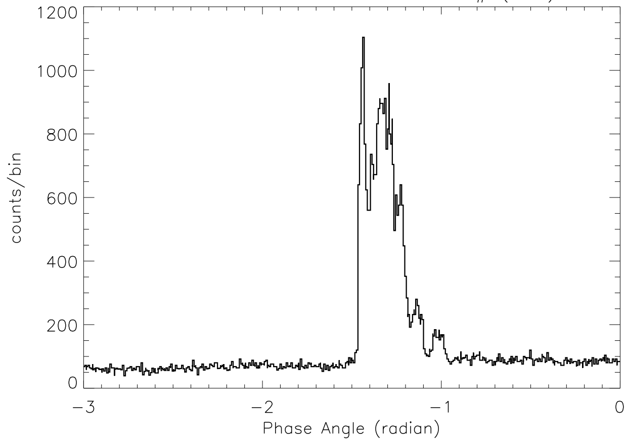
SOX2: 23: 5:56 – 23: 6: 5 SP# ( 80)
