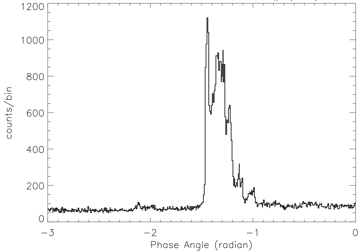
SOX2: 23: 5:12 – 23: 5:21 SP# ( 75)
