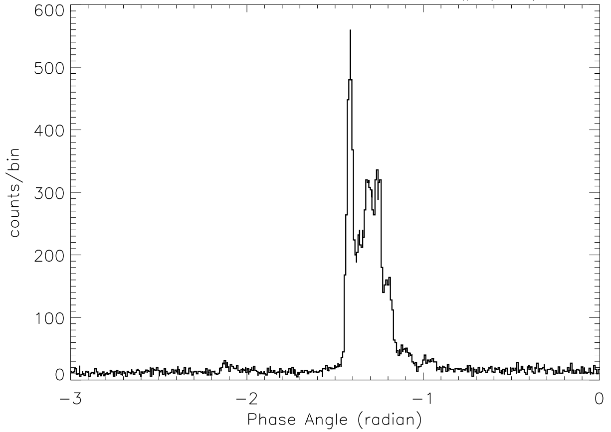
SOX2: 22:56:39 – 22:56:48 SP# ( 16)
