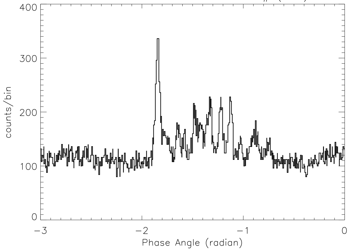
SOX2: 23: 5:56 – 23: 6: 5 SP# ( 80)
