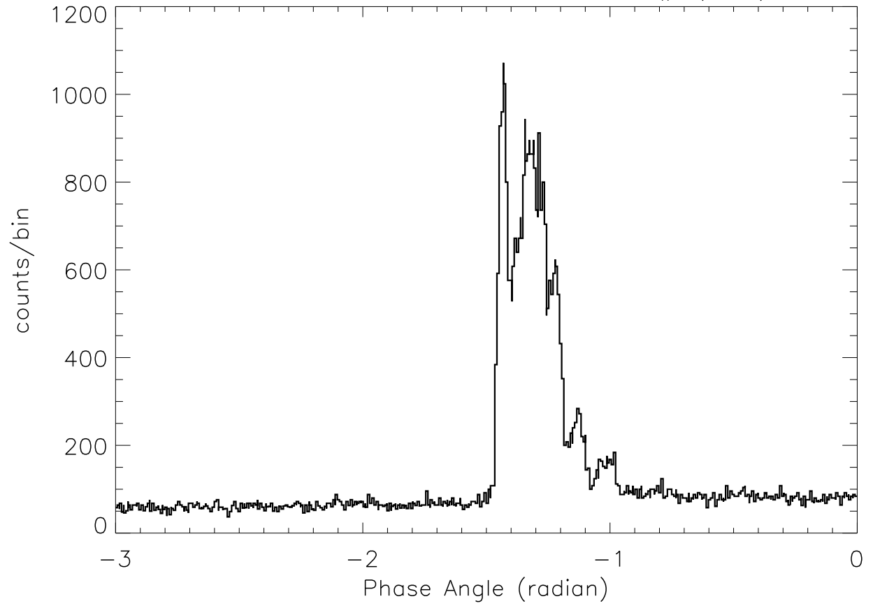
SOX2: 23: 6:31 – 23: 6:39 SP# ( 84)
