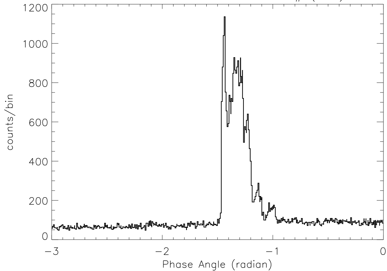
SOX2: 23: 5:30 – 23: 5:38 SP# ( 77)
