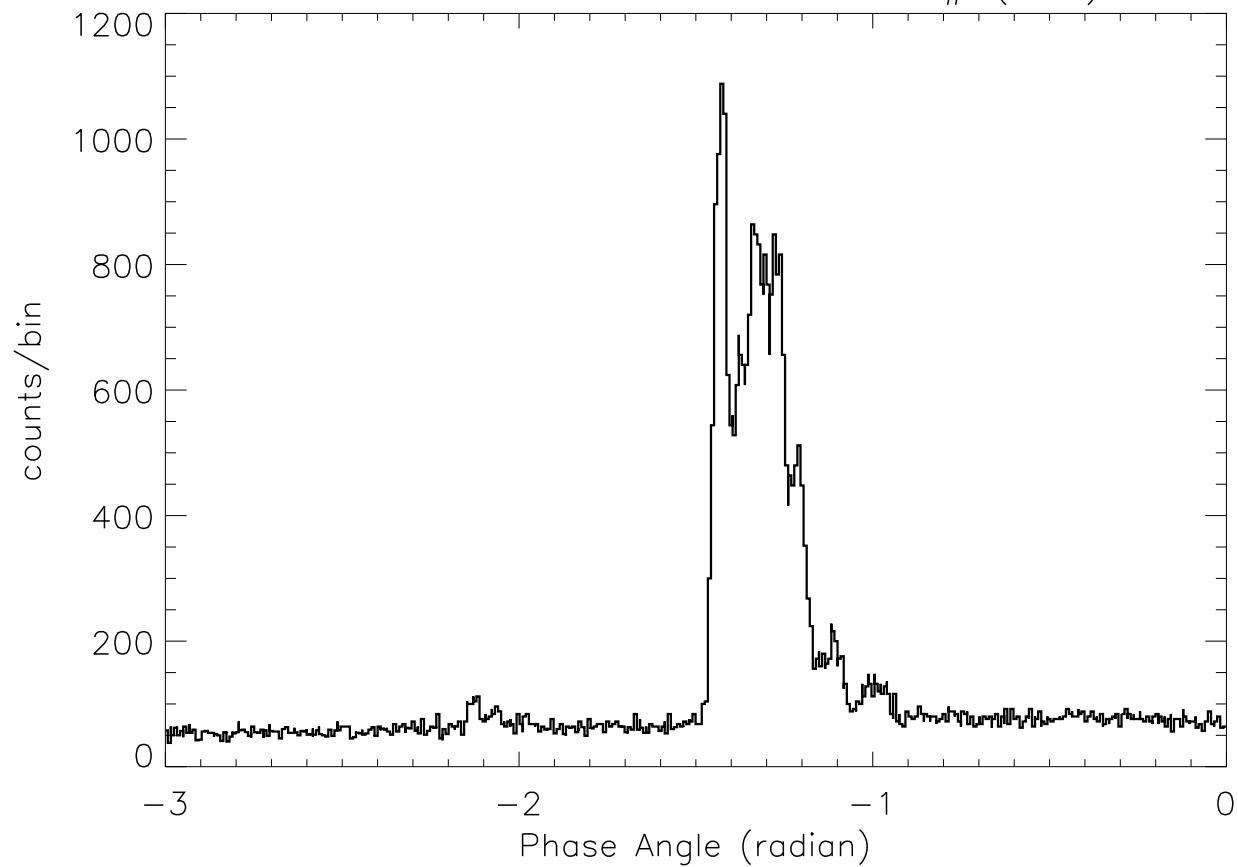
SOX2: 23: 1:35 – 23: 1:44 SP# ( 50)
