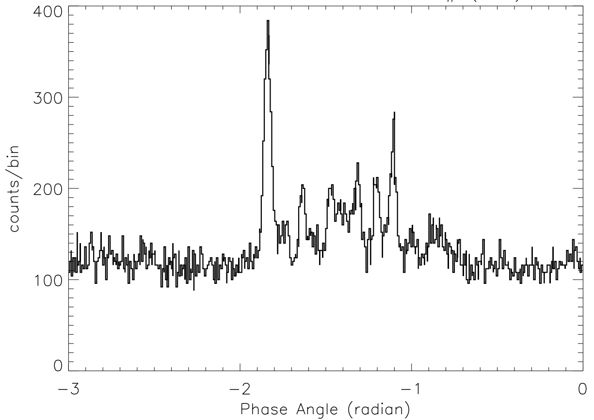
SOX2: 23: 3:11 – 23: 3:19 SP# ( 61)
