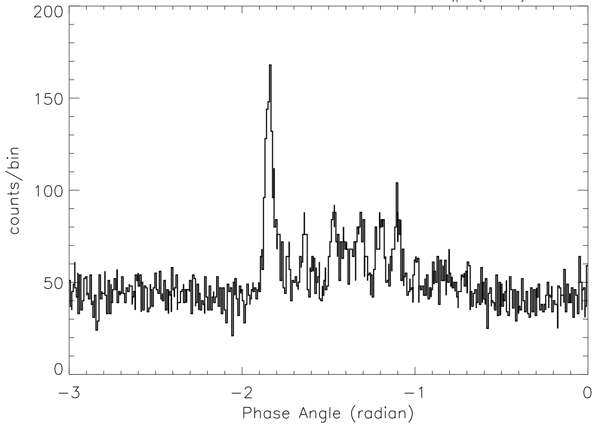
SOX2: 22:58: 6 – 22:58:15 SP# ( 26)
