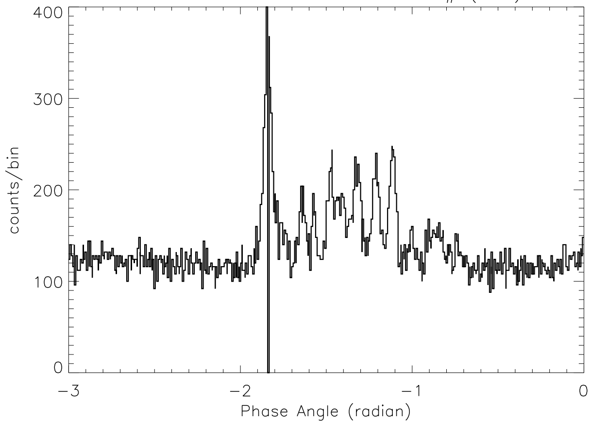
SOX2: 23: 3:54 – 23: 4: 3 SP# ( 66)
