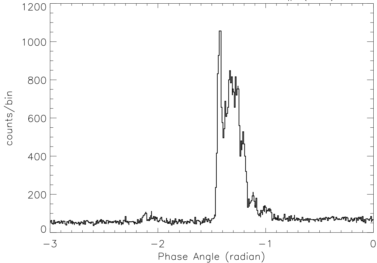
SOX2: 23: 1:18 – 23: 1:26 SP# ( 48)
