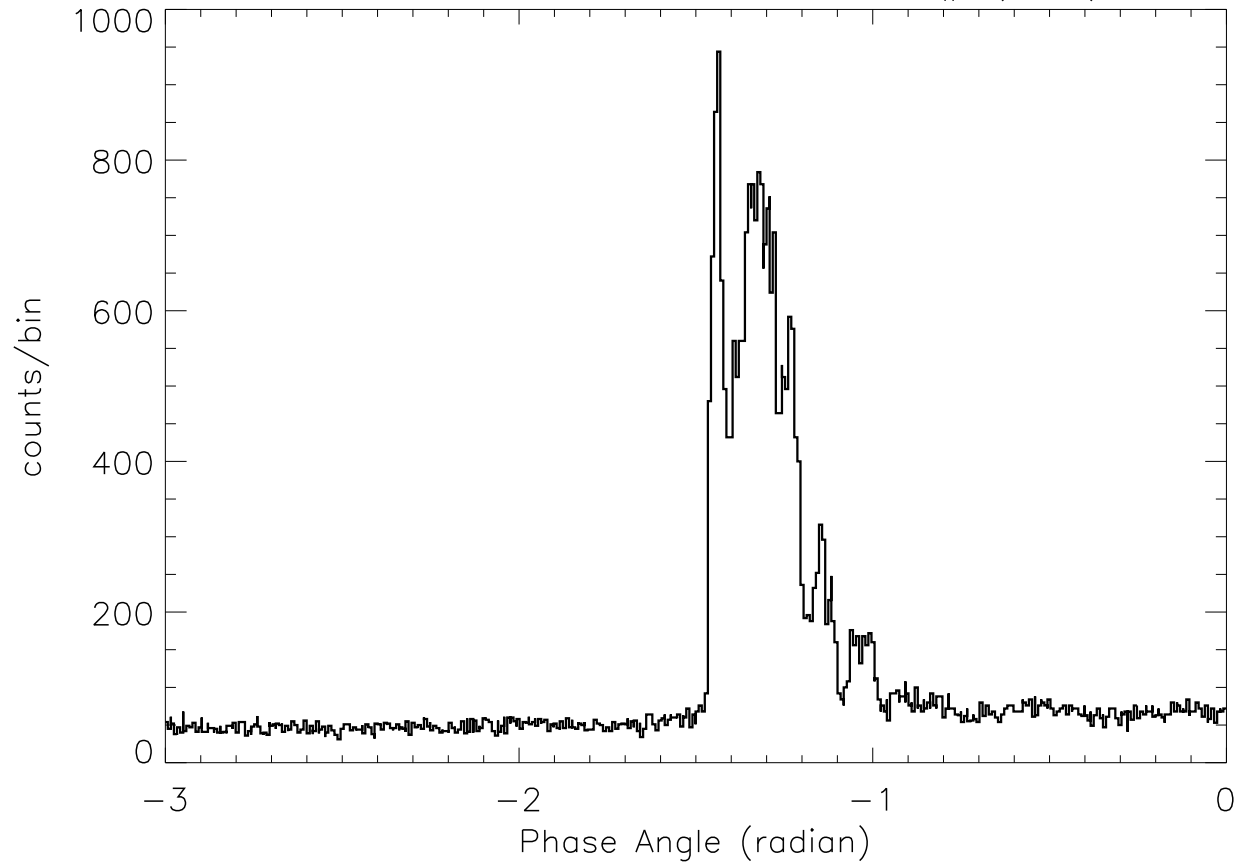
SOX2: 23: 9:42 – 23: 9:51 SP# (106)
