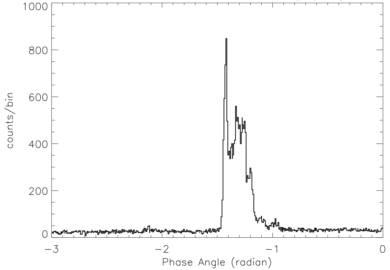
SOX2: 22:58: 6 – 22:58:15 SP# ( 26)
