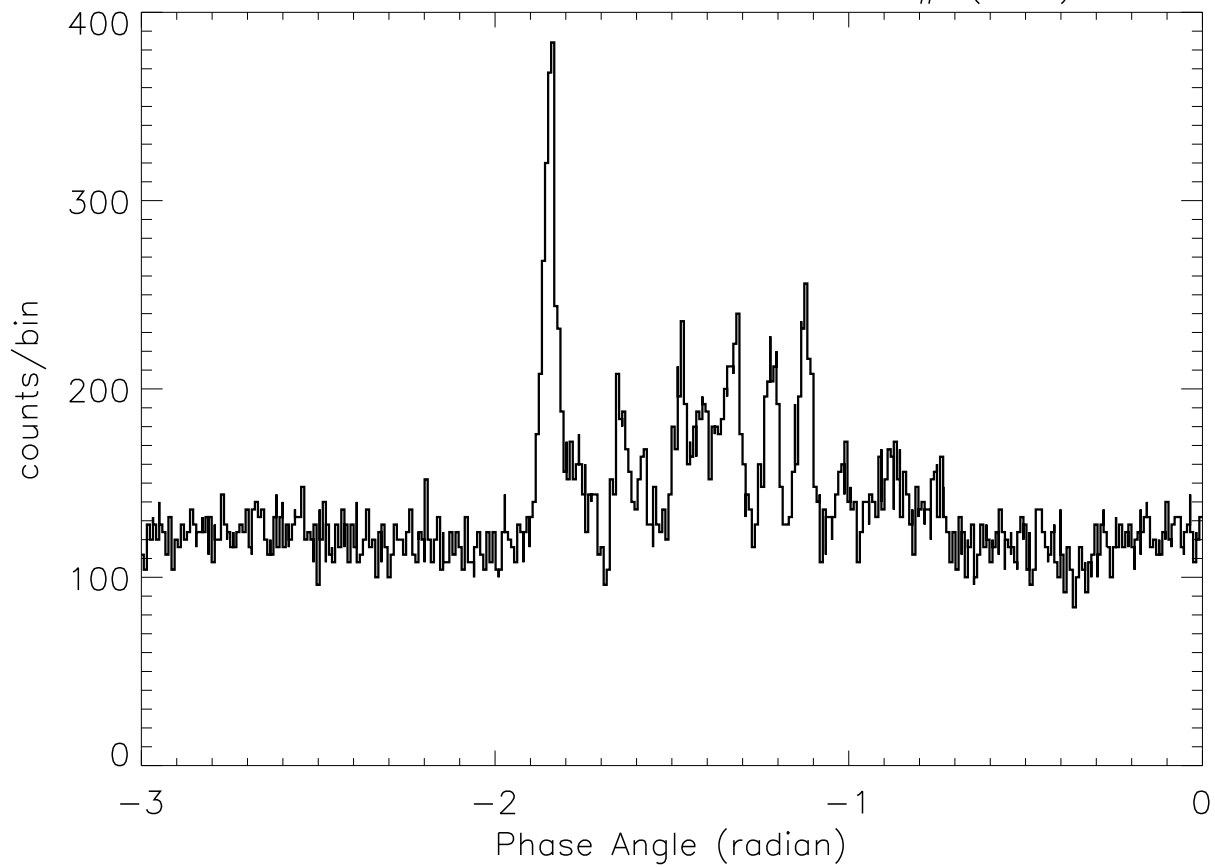
SOX2: 23: 4:55 – 23: 5: 4 SP# ( 73)
