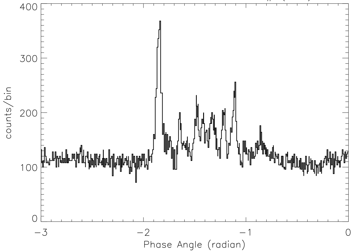
SOX2: 23: 2:36 – 23: 2:45 SP# ( 57)
