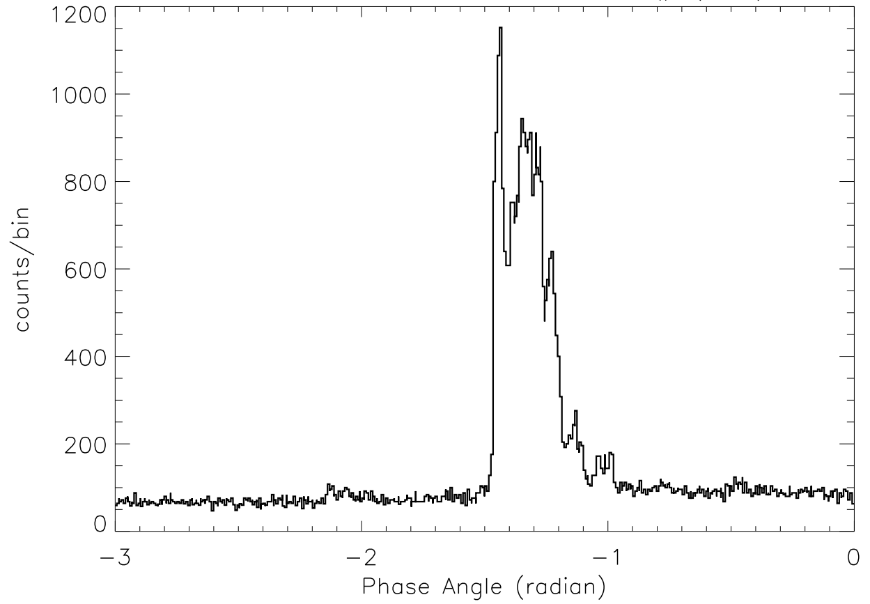
SOX2: 23: 4:29 – 23: 4:38 SP# ( 70)
