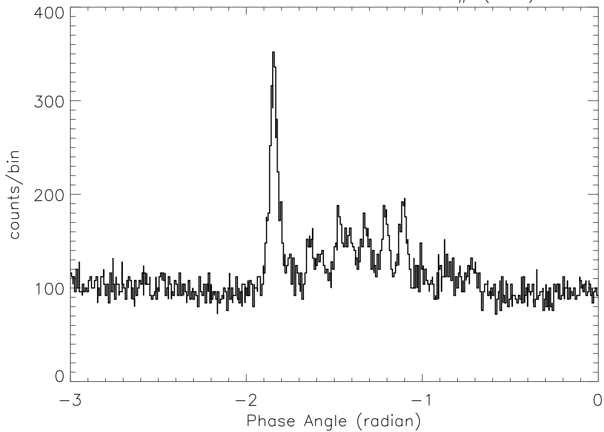
SOX2: 23: 1:35 – 23: 1:44 SP# ( 50)
