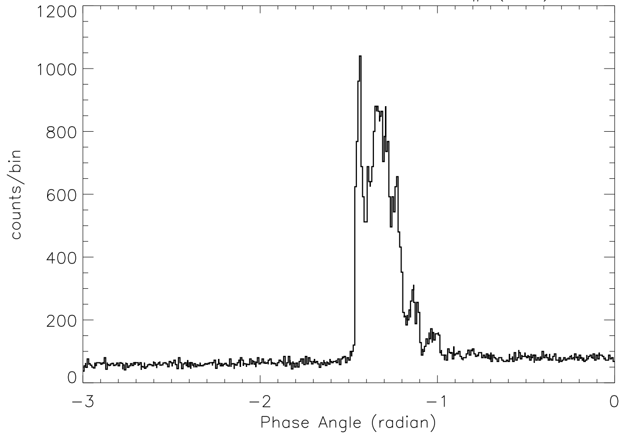
SOX2: 23: 7: 5 – 23: 7:14 SP# ( 88)
