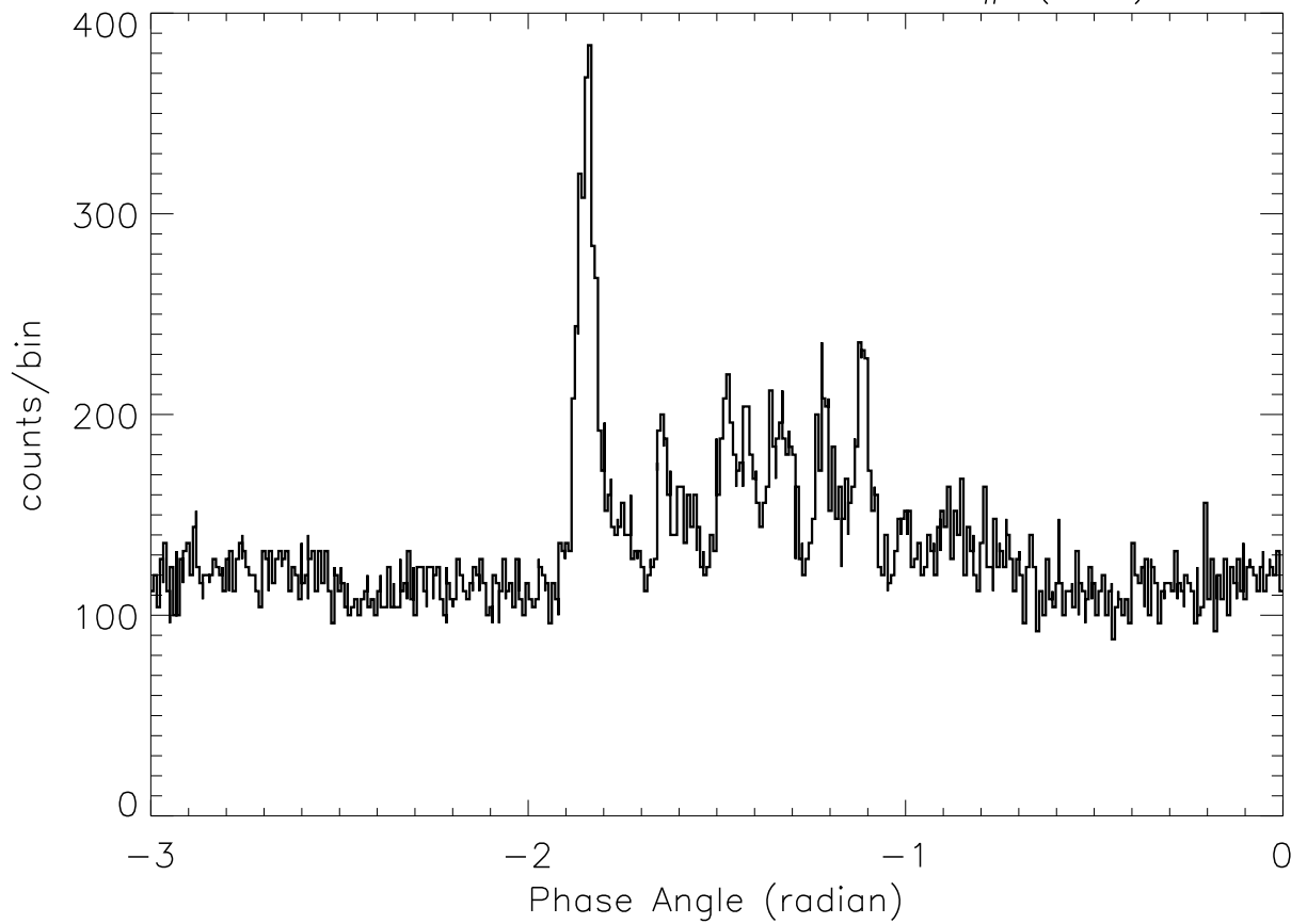
SOX2: 23: 3:19 – 23: 3:28 SP# ( 62)
