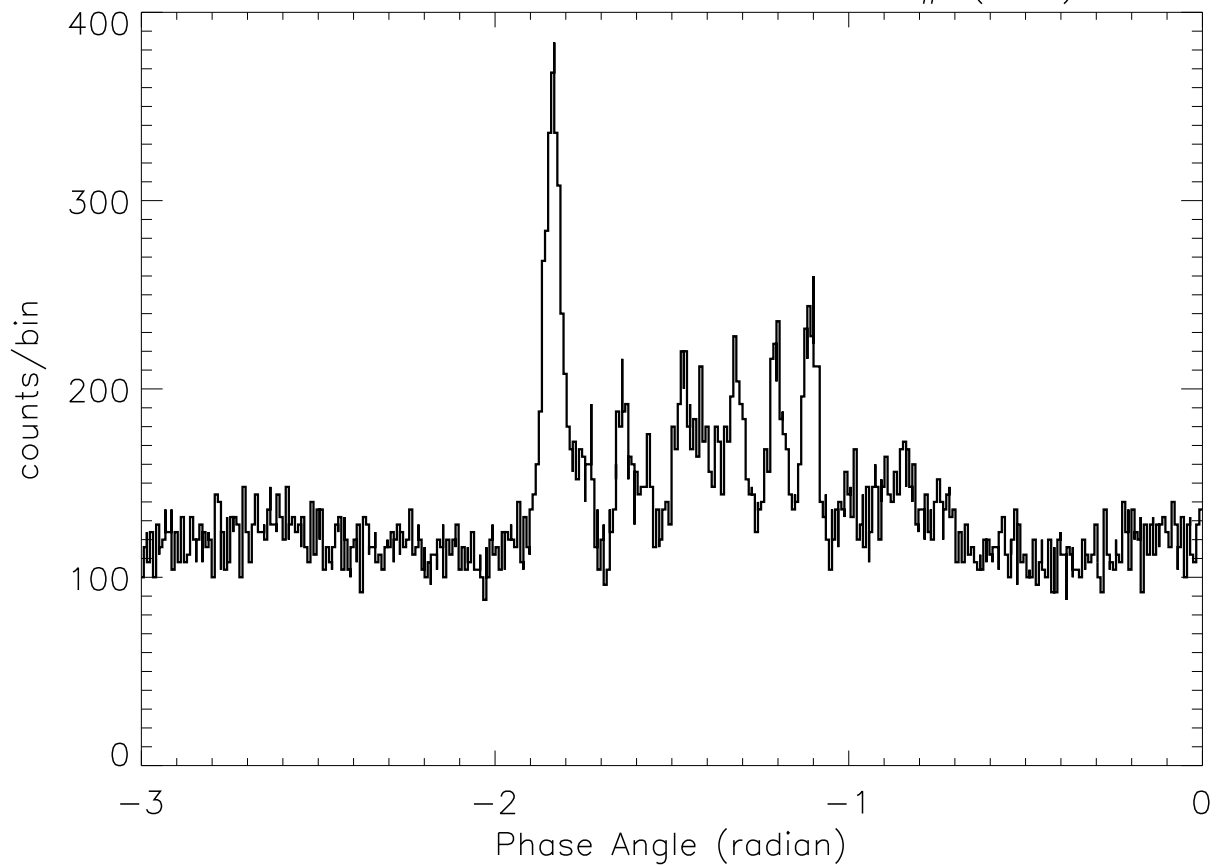
SOX2: 23: 3:28 – 23: 3:37 SP# ( 63)
