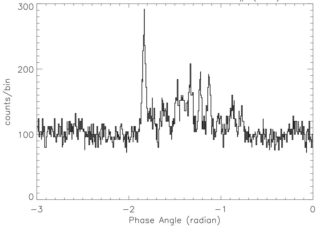
SOX2: 23: 8:24 – 23: 8:32 SP# ( 97)
