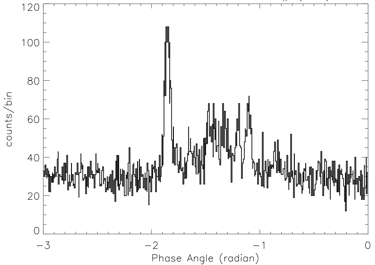
SOX2: 22:57: 5 – 22:57:14 SP# ( 19)
