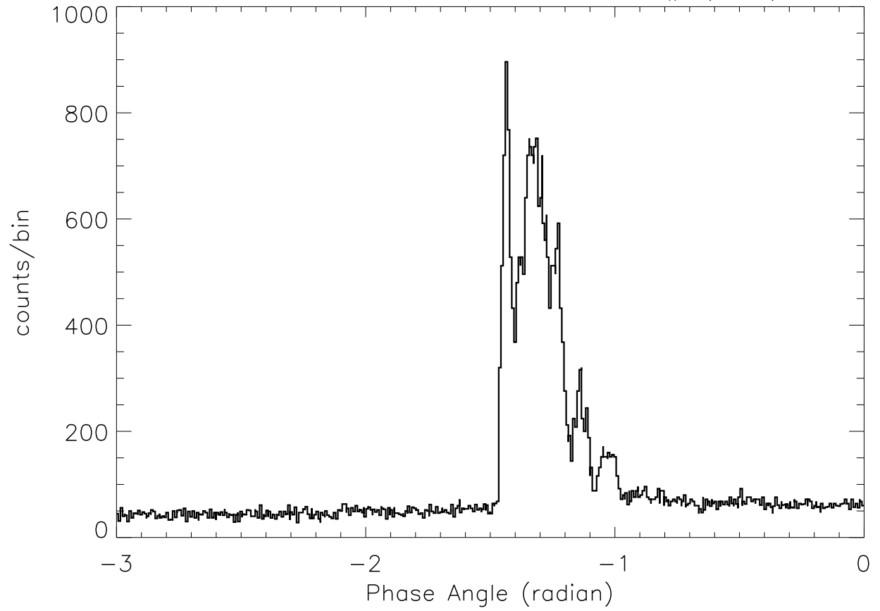
SOX2: 23:10:17 – 23:10:25 SP# (110)
