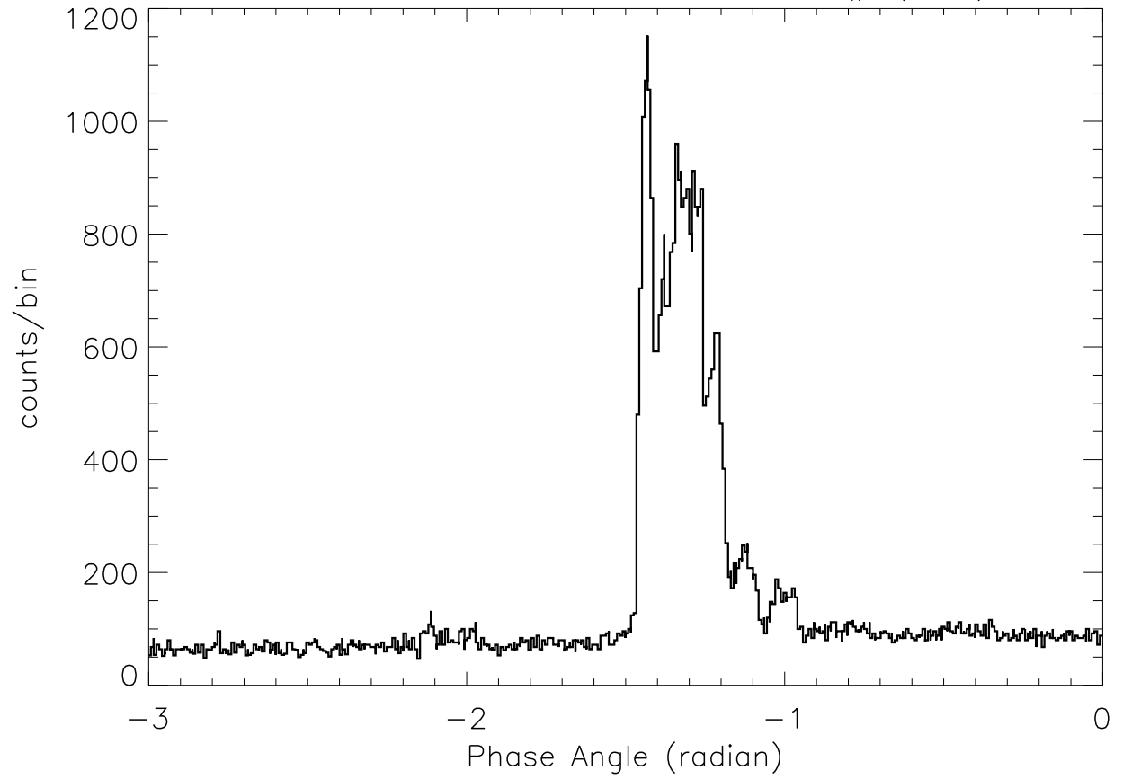
SOX2: 23: 3:45 – 23: 3:54 SP# ( 65)
