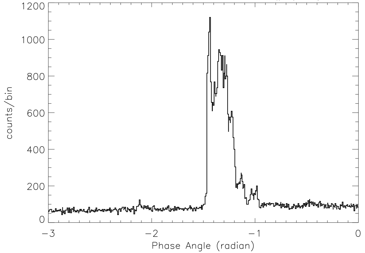
SOX2: 23: 4:11 – 23: 4:20 SP# ( 68)
