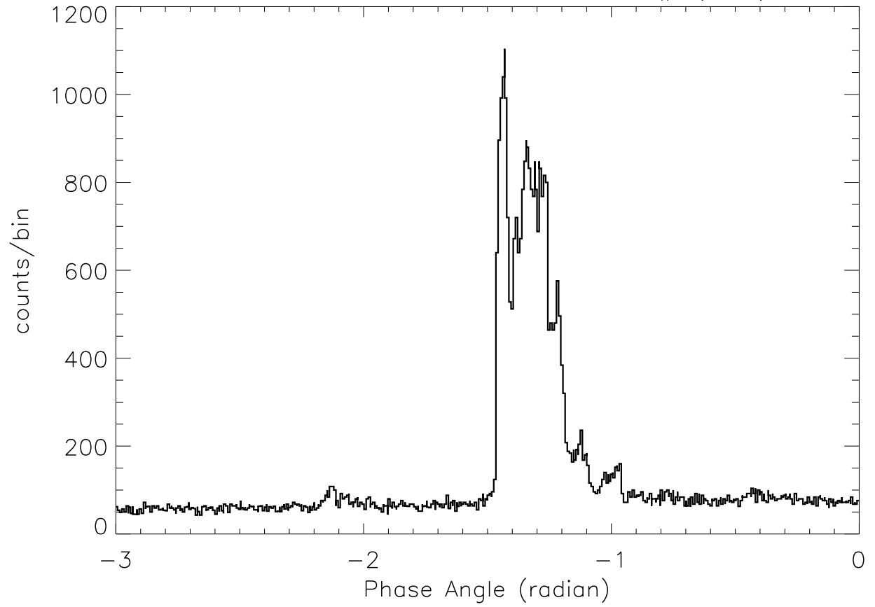
SOX2: 23: 1:52 - 23: 2: 1 SP# ( 52)
