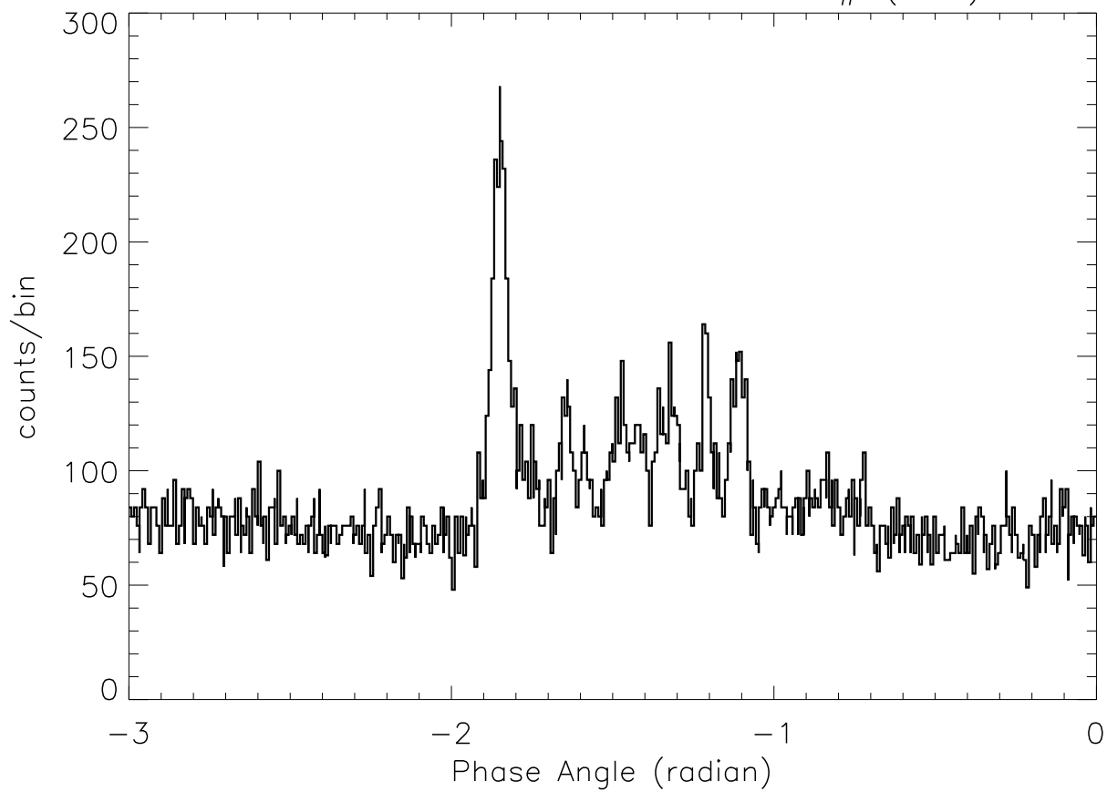
SOX2: 23: 0:25 – 23: 0:34 SP# ( 42)
