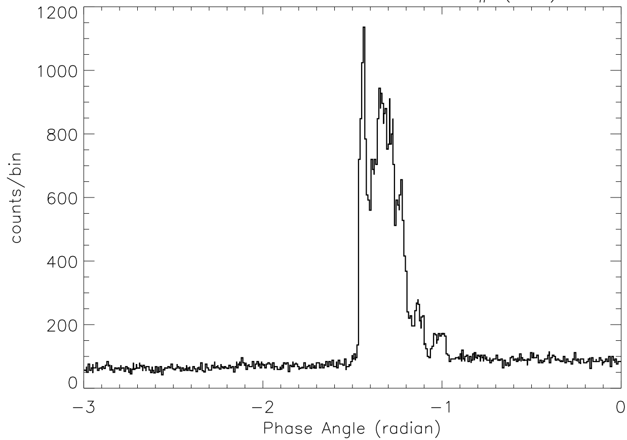
SOX2: 23: 5:38 – 23: 5:47 SP# ( 78)
