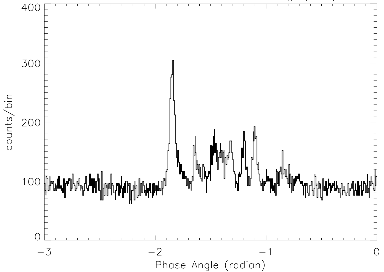
SOX2: 23: 1: 9 - 23: 1:18 SP# ( 47)
