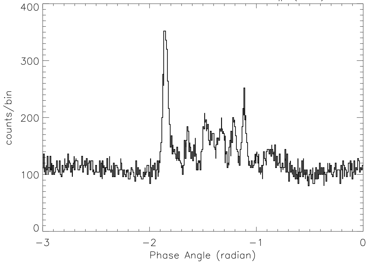
SOX2: 23: 2:27 – 23: 2:36 SP# ( 56)
