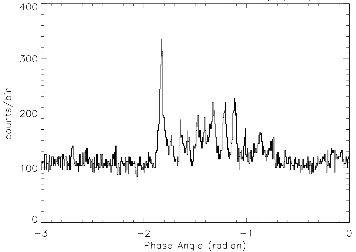
SOX2: 23: 6:39 – 23: 6:48 SP# ( 85)
