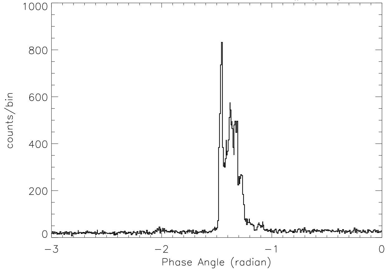
SOX2: 4:35:50 – 4:35:58 SP# ( 31)
