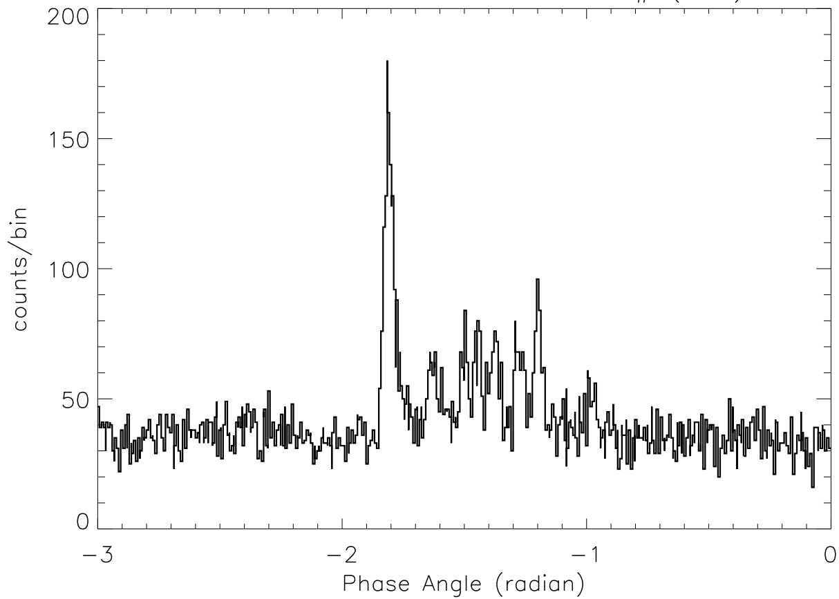
SOX2: 4:35:32 – 4:35:41 SP# ( 29)
