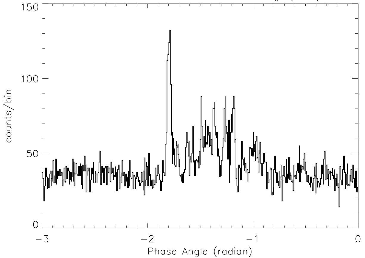
SOX2: 4:37:35 - 4:37:44 SP# ( 43)
