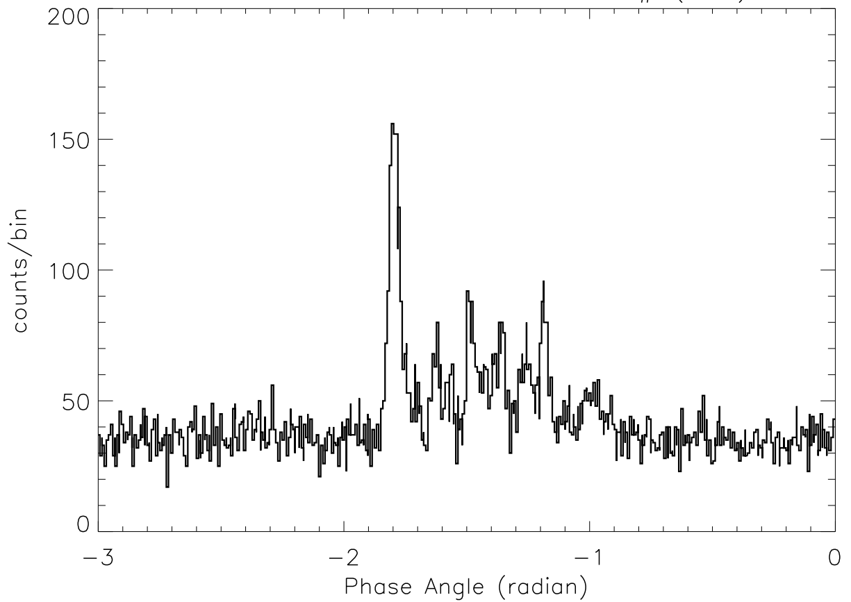
SOX2: 4:35:41 – 4:35:50 SP# ( 30)
