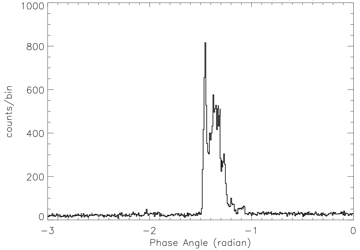
SOX2: 4:36: 7 - 4:36:16 SP# ( 33)
