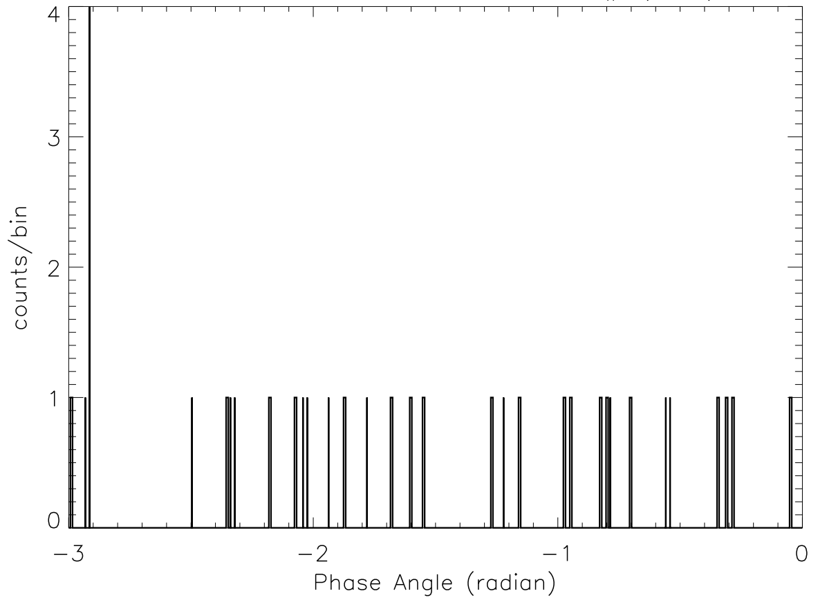
SOX2: 4:46:49 – 4:46:58 SP# (106)
