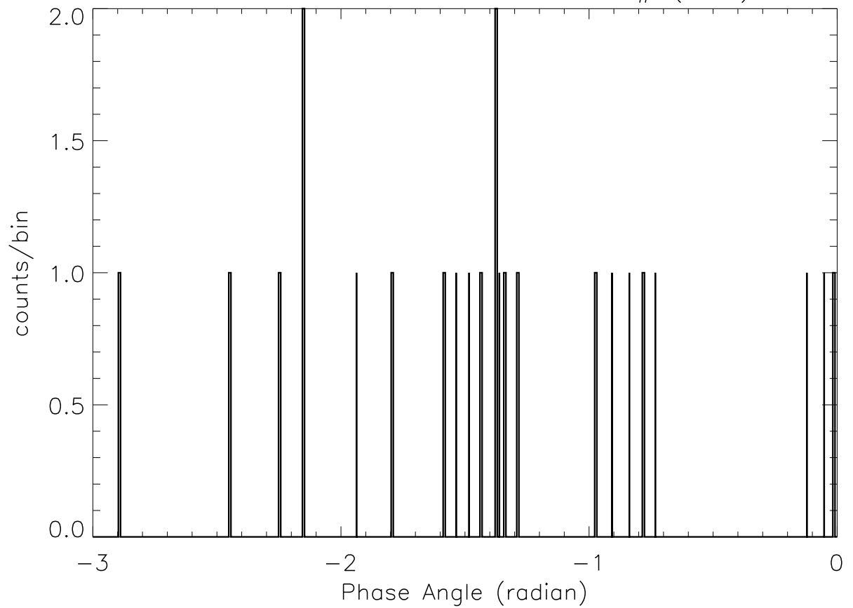
SOX2: 4:47:24 – 4:47:33 SP# (110)
