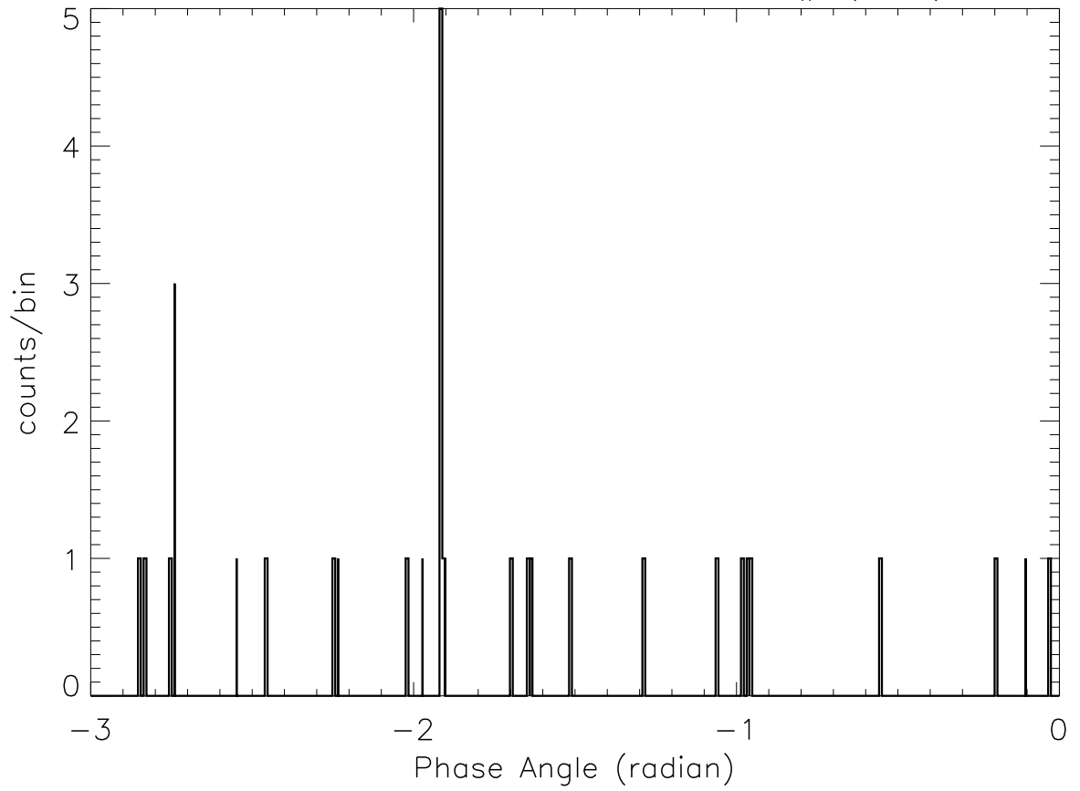
SOX2: 4:47:24 – 4:47:33 SP# (110)
