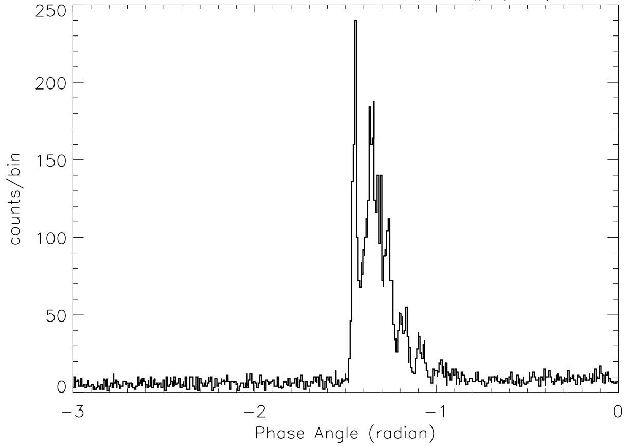
SOX2: 4:40:40 – 4:40:49 SP# ( 64)
