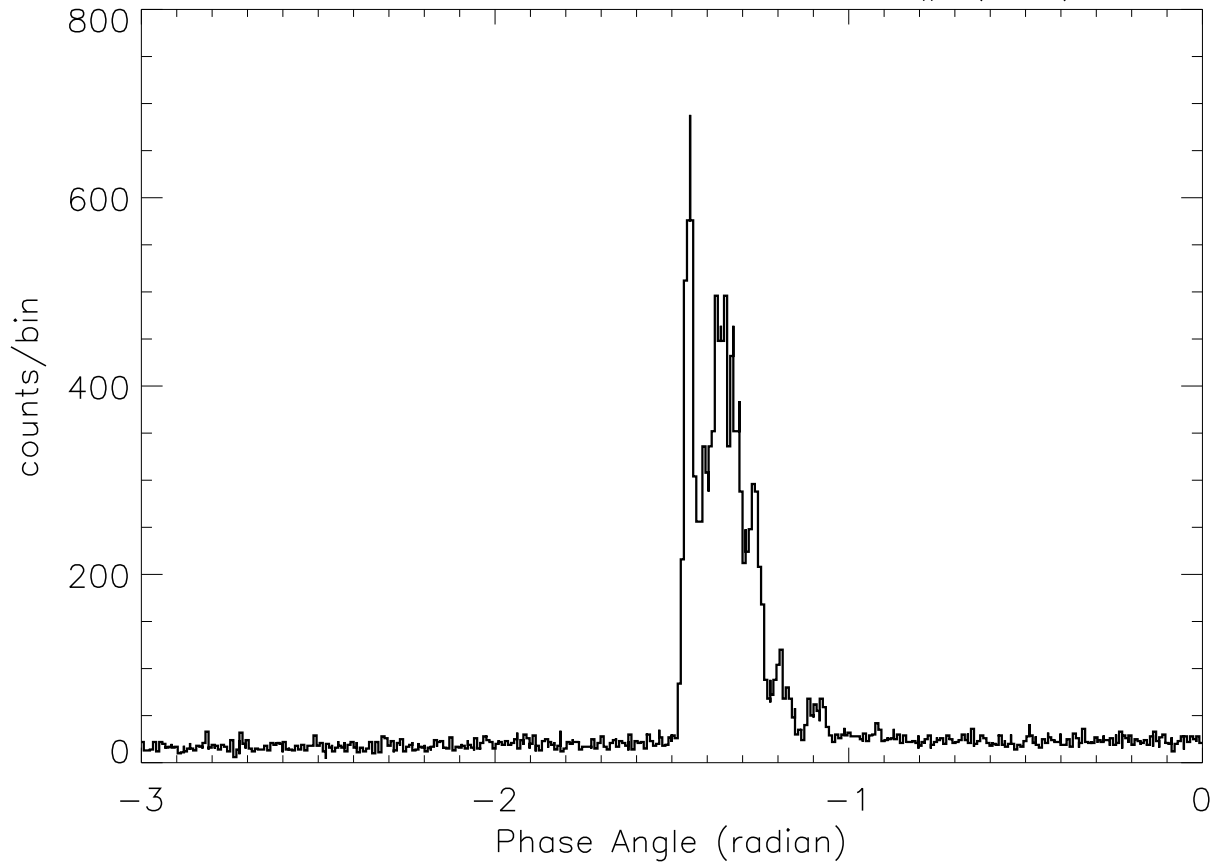
SOX2: 4:37:44 – 4:37:53 SP# ( 44)
