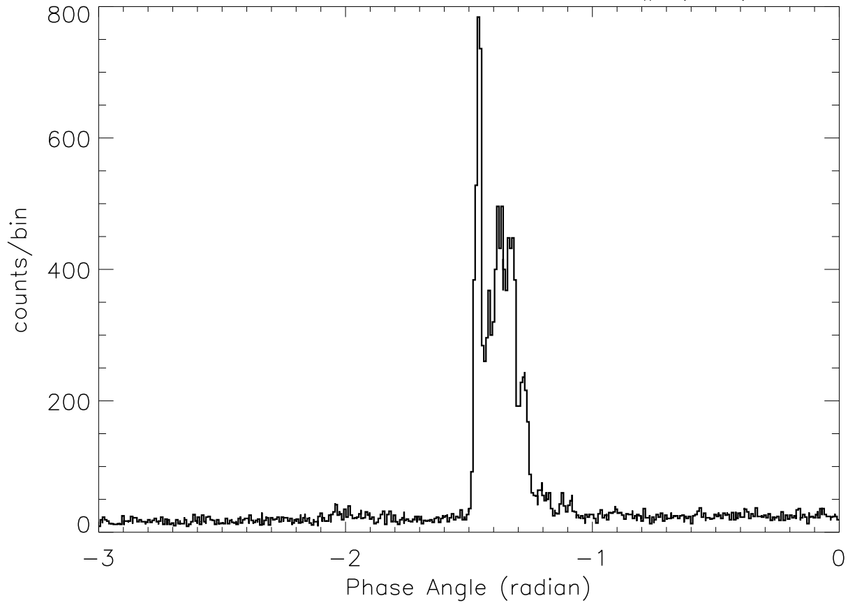
SOX2: 4:35:23 - 4:35:32 SP# ( 28)
