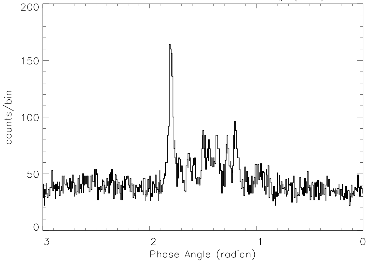
SOX2: 4:35:50 – 4:35:58 SP# ( 31)
