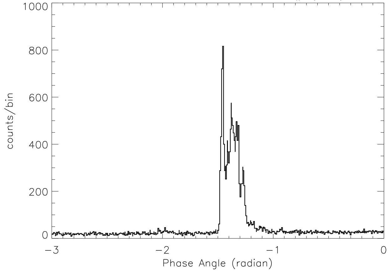
SOX2: 4:35:41 – 4:35:50 SP# ( 30)
