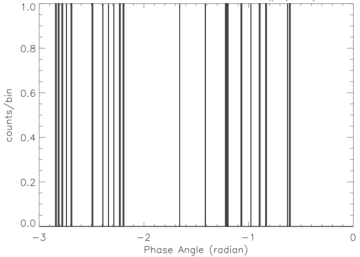
SOX2: 4:46:49 – 4:46:58 SP# (106)
