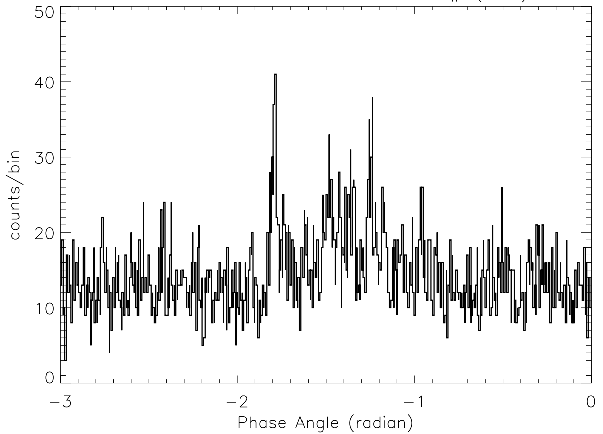
SOX2: 4:40:40 – 4:40:49 SP# ( 64)
