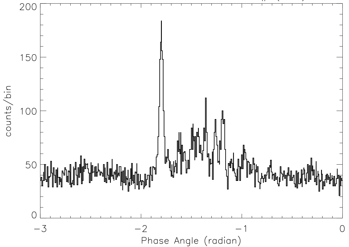
SOX2: 4:36: 7 - 4:36:16 SP# ( 33)
