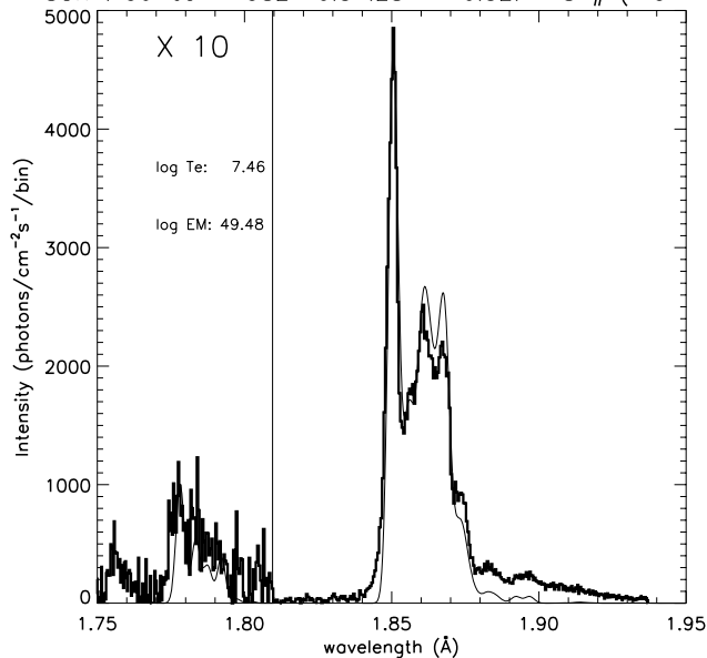
SOX1: 06-Jun-1982 16:32:44 – 16:34: 0 SP# ( 17– 24)
