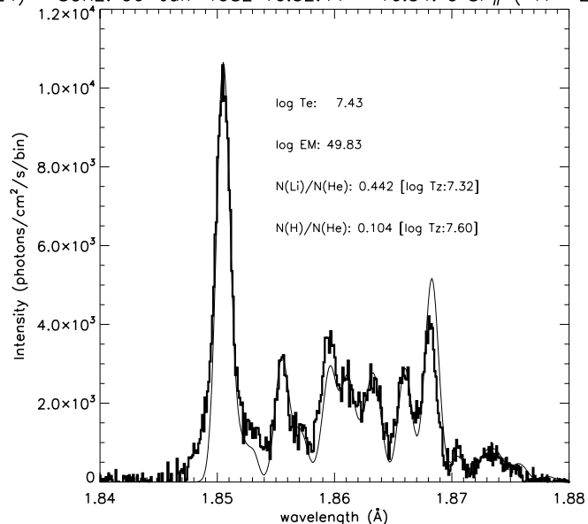
SOX2: 06-Jun-1982 16:34: 0 – 16:35:15 SP# ( 25– 32)
