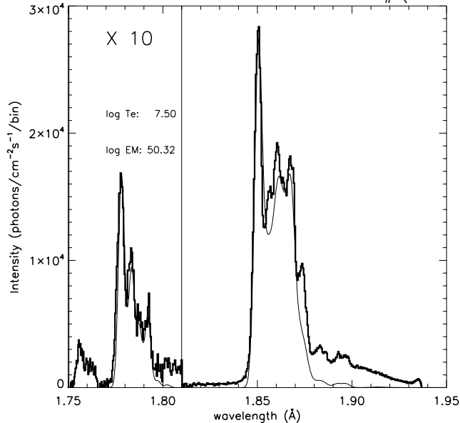
SOX1: 06-Jun-1982 16:34: 0 – 16:35:15 SP# ( 25– 32)
