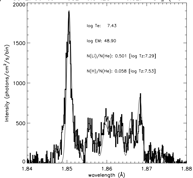
SOX2: 06-Jun-1982 16:32:44 – 16:34: 0 SP# ( 17– 24)
