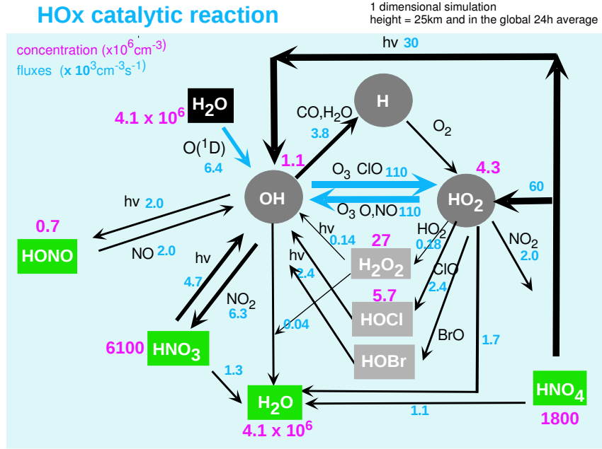
Figure 2.8 Gas phase reaction of HO x in the stratosphere (Based on Brasseur [2000]).
