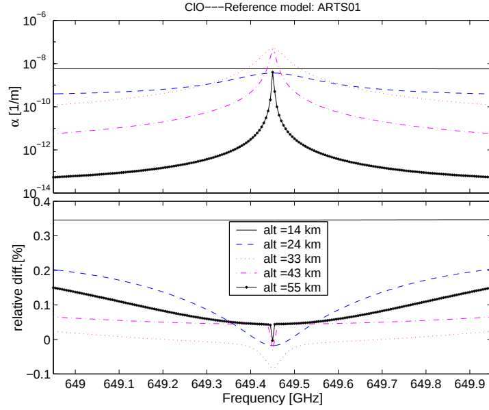
Figure 4.6 Upper: ARTS calculations of the absorption spectra in the frequency range around the ClO line at 649.45 GHz for different atmospheric levels. Lower: Relative difference between the absorption spectra calculated with the two models SMOCO and ARTS. The ARTS model was taken as a reference model.
