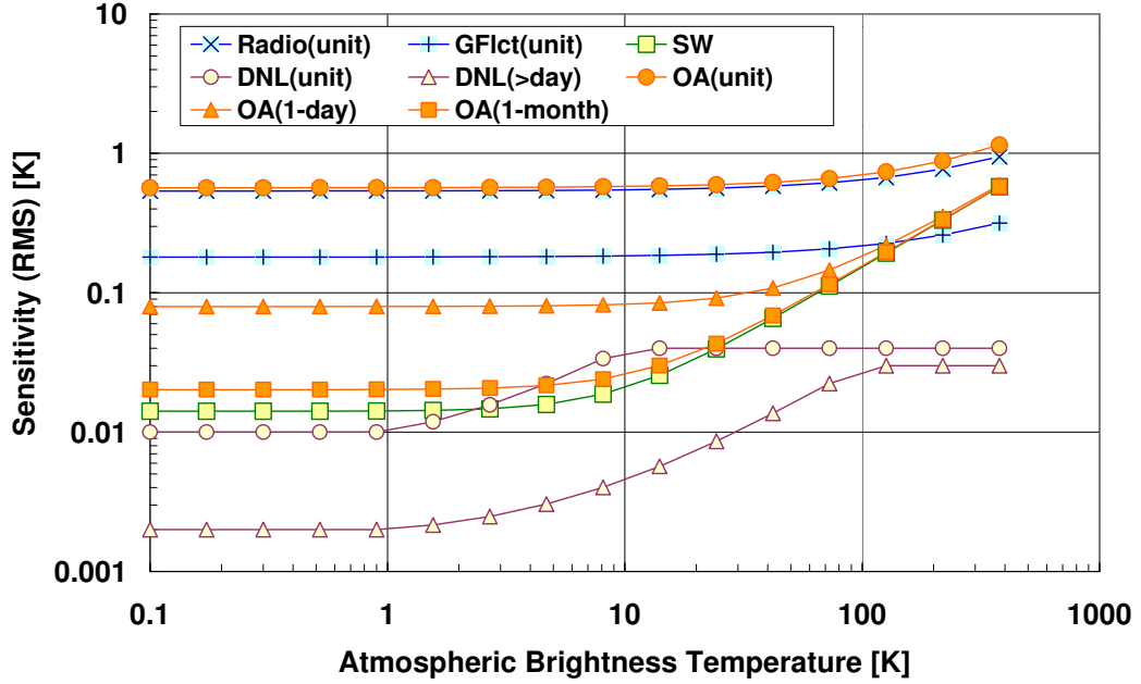
Figure 3.41 Overall Sensitivity: “Radio”; radiometric noise, “GFlct”; gain fluctuation, “SW”; standing waves, “DNL”; differential non-linearity of the analog-to-digital converter, “OA”; overall sensitivity obtained by rss (root-sum-squares). “unit” means the unit data obtained in 53 seconds. Standing waves are not reduced by averaging.
