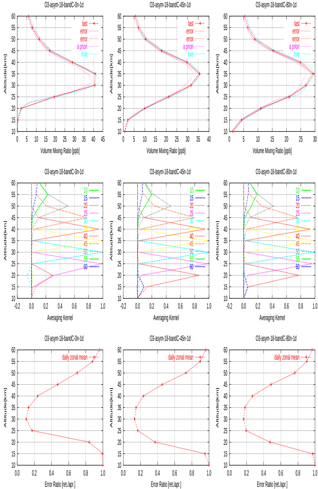
Figure A.12 Retrieval simulation results for 30-scan averaged data in BAND-C for asymmetric-18 ozone at latitudes of 0°N (left), 45°N (center), and 80°N (right). Top: Retrieved volume mixing ratios are shown with rms retrieval error bounds and a priori profiles which are here assumed to be 90% of the true profile; Middle Averaging kernels; Bottom: Retrieval error ratios defined as the ratio of the retrieval errors to the a priori errors which are assumed to be 10 % of the a priori volume mixing ratios.
