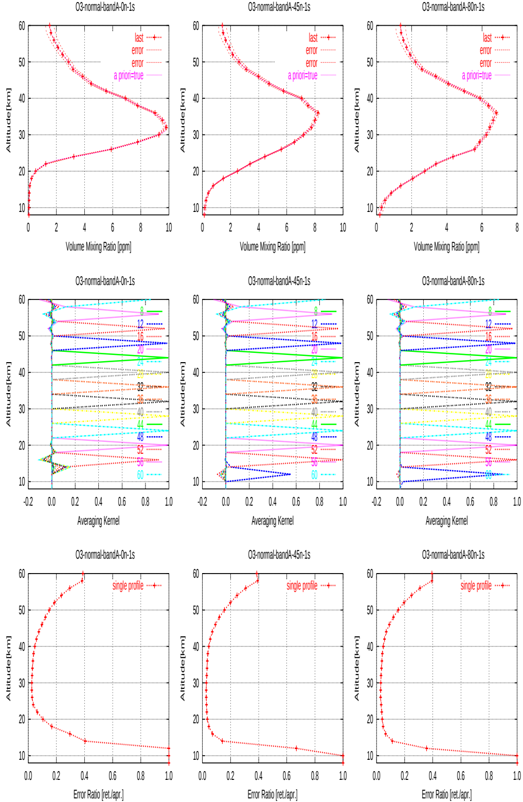
Figure A.1 Retrieval simulation results for single-scan data in BAND-A for standard profiles of normal O 3 at latitudes of 0°N (left), 45°N (center), and 80°N (right). Top: Retrieved volume mixing ratios are shown with rms retrieval error bounds and a priori profiles which are assumed to coincide with true profiles; Middle Averaging kernels; Bottom: Retrieval error ratios defined as the ratio of the retrieval errors to the a priori errors which are assumed to be 50 % of the a priori volume mixing ratios.
