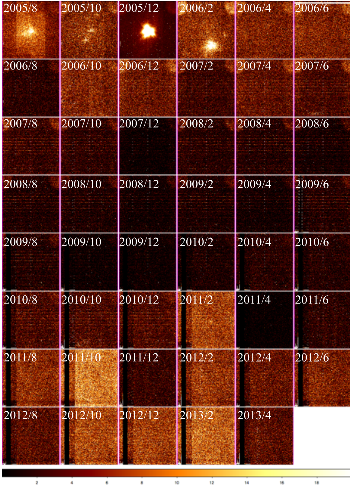
Figure 2: DYE images of XIS0 integrated for two month intervals from 2005 Aug–Sept to 2013 Apr–May. Events with the grade 0, 2, 3, 4, or 6 were used. The first four images should be ignored as they erroneously include some X-ray sources.
